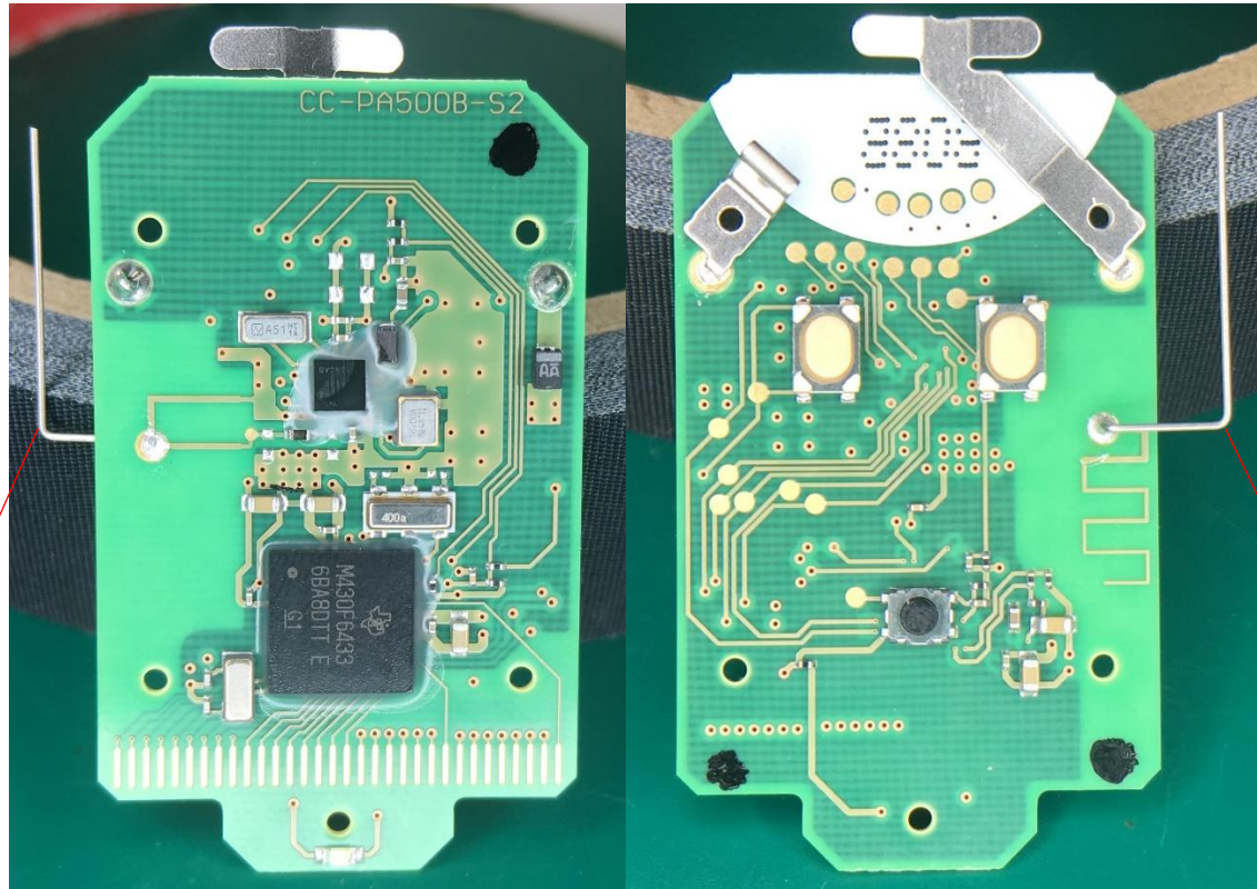
Lead Antenna
