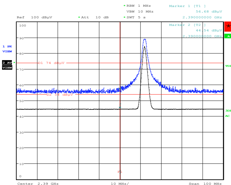
Figure 14: Radiated Emissions at Band Edge, Spectral Diagram, Mode A (2402MHz)
