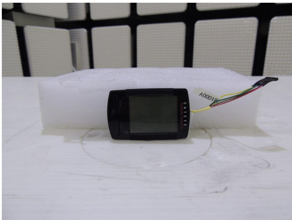
Photograph 5: Set-up for Radiated Emission, EUT Configuration Y-Axis at 80cm height
