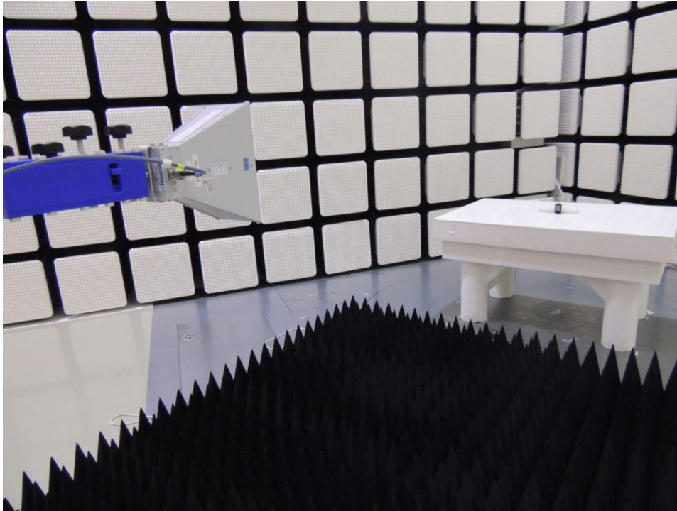
Photograph 2: Set-up for Radiated Emission of Transmitter, Measuring Antenna View at 80cm height
