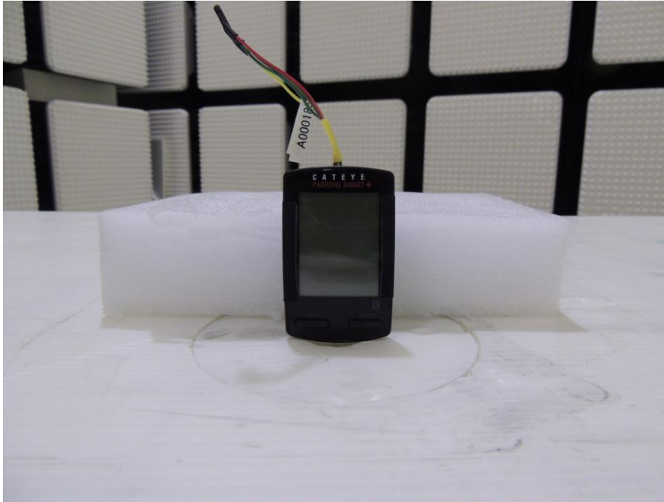
Photograph 6: Set-up for Radiated Emission, EUT Configuration Z-Axis at 80cm height
