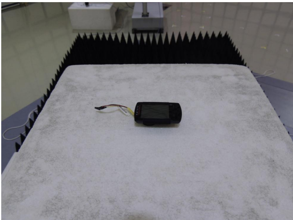
Photograph 3: Set-up for Radiated Emission of Transmitter, Measuring Antenna View at 1.5m height
