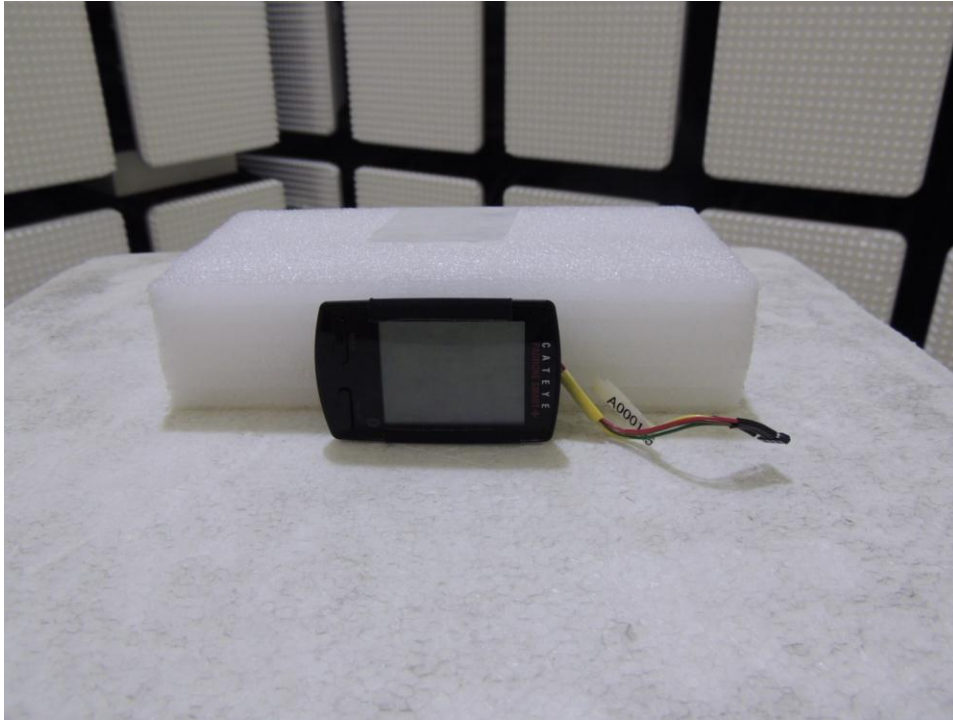
Photograph 8: Set-up for Radiated Emission, EUT Configuration Y-Axis at 1.5m height
