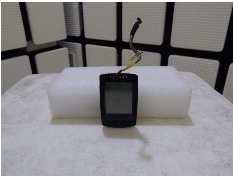
Photograph 9: Set-up for Radiated Emission, EUT Configuration Z-Axis at 1.5m height
