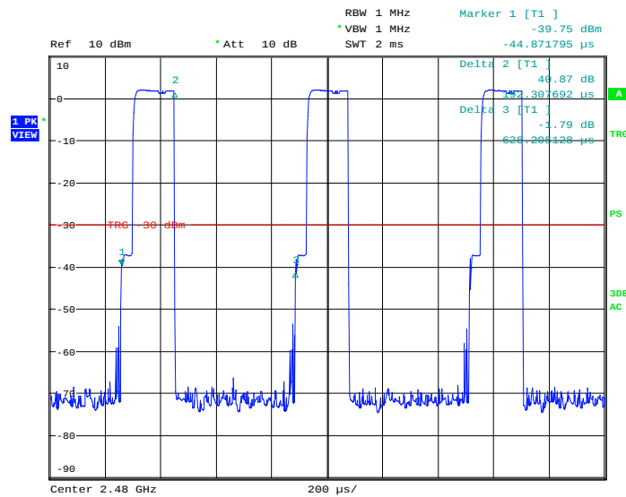
Figure 4: Duty Cycle, Mode C (2480MHz)
