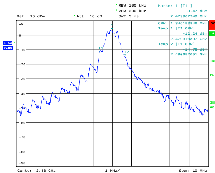
Figure 10: 99% Bandwidth, Mode C (2480MHz)
