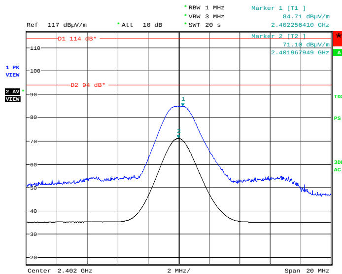
Figure 11: Field Strength of Fundamental, Spectral Diagram, Mode A (2402MHz)
