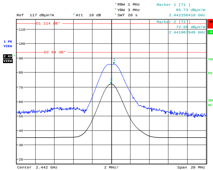
Figure 12: Field Strength of Fundamental, Spectral Diagram, Mode B (2442MHz)
