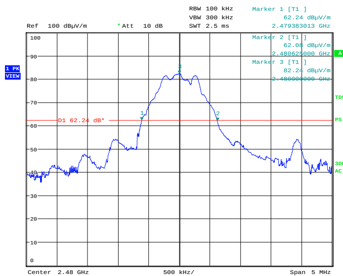
Figure 6: 20dB Bandwidth, Mode C (2480MHz)
