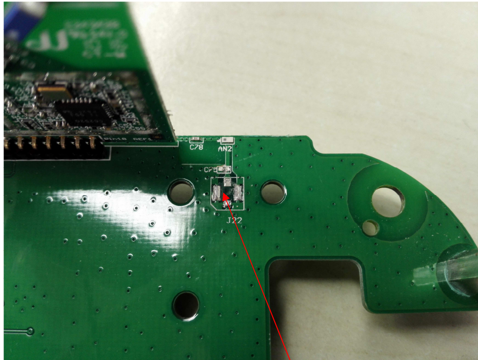
RF base for antenna 2
