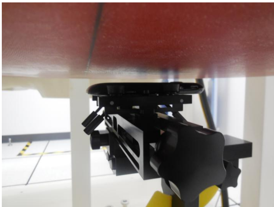
Band850, Band1900 Test Setup Body Back with gap 10mm
