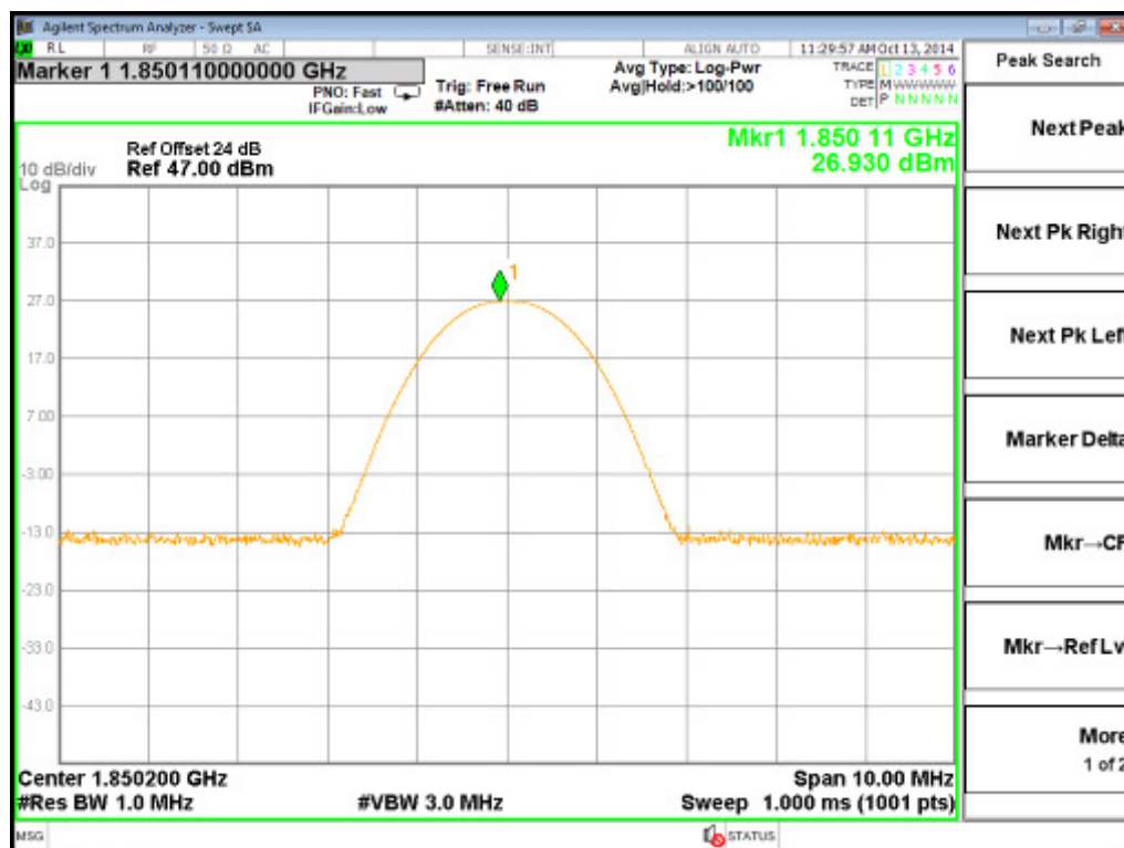
Channel 512
