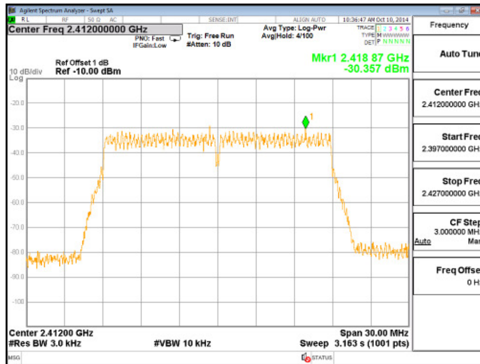
Channel 01 (2412MHz)
