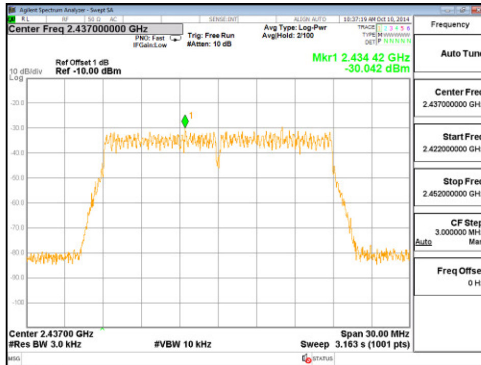
Channel 06 (2437MHz)
