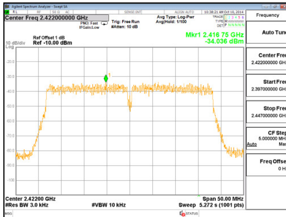
Channel 03 (2422MHz)
