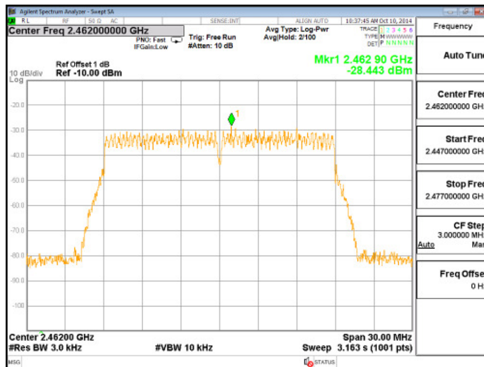
Channel 11 (2462MHz)
