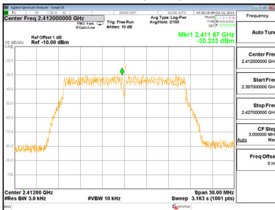
Channel 01 (2412MHz)
