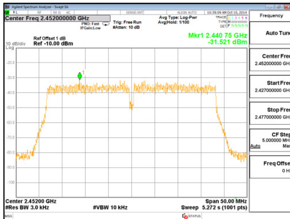
Channel 09 (2452MHz)
