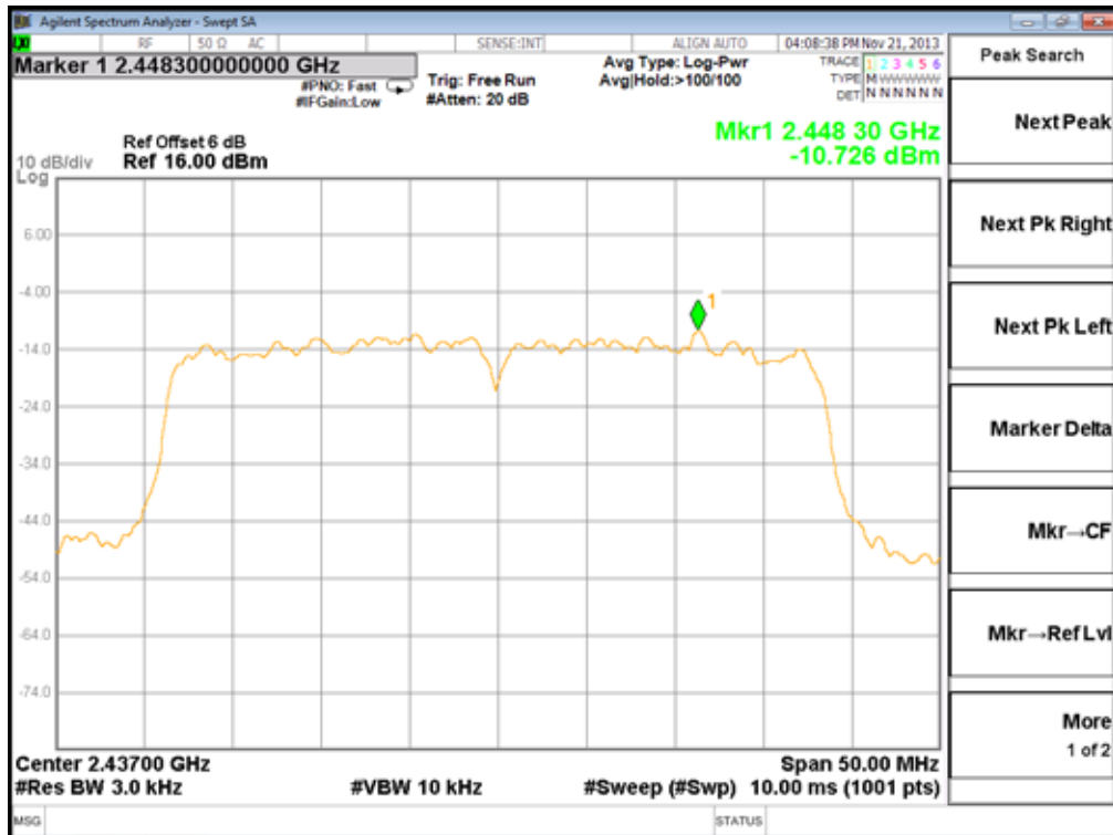
Channel 06 (2437MHz)
