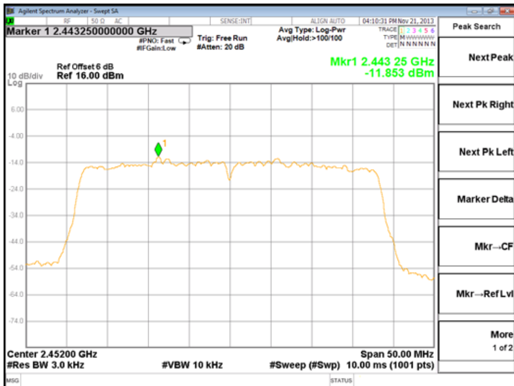
Channel 09 (2452MHz)
