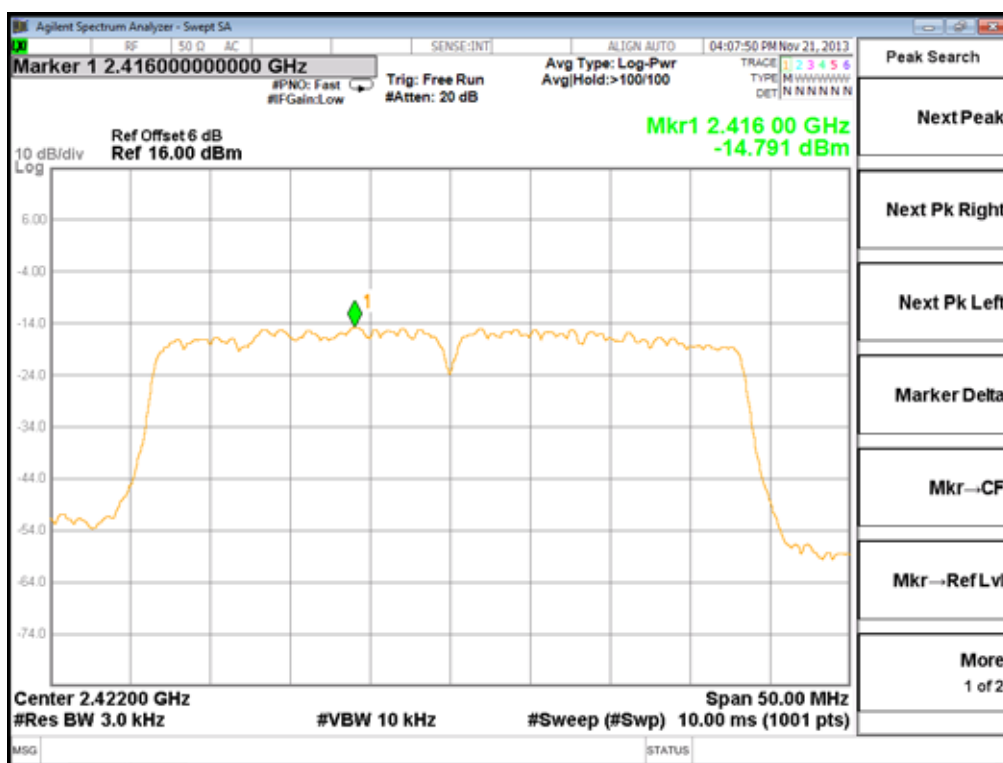
Channel 03 (2422MHz)
