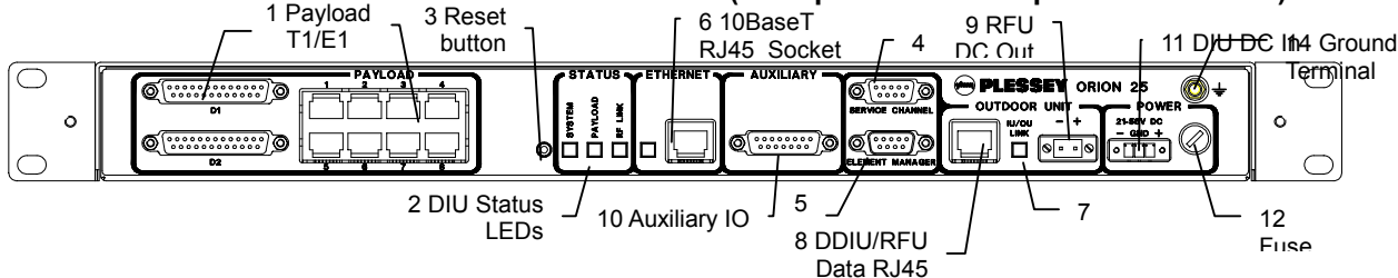
Figure 5. Digital Indoor Unit Connector Panels.
