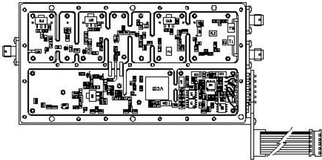
Rx Housing Assembly Open
