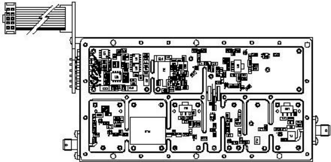
Tx Housing Assembly Open
