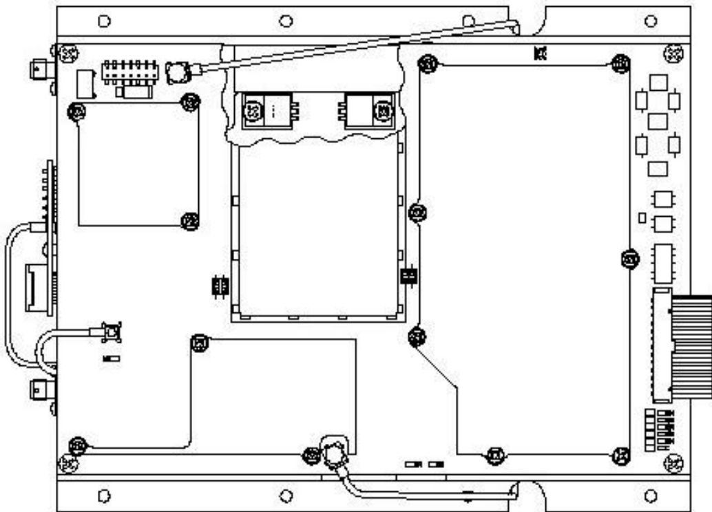
Baseband Processor Assembly with Cans
