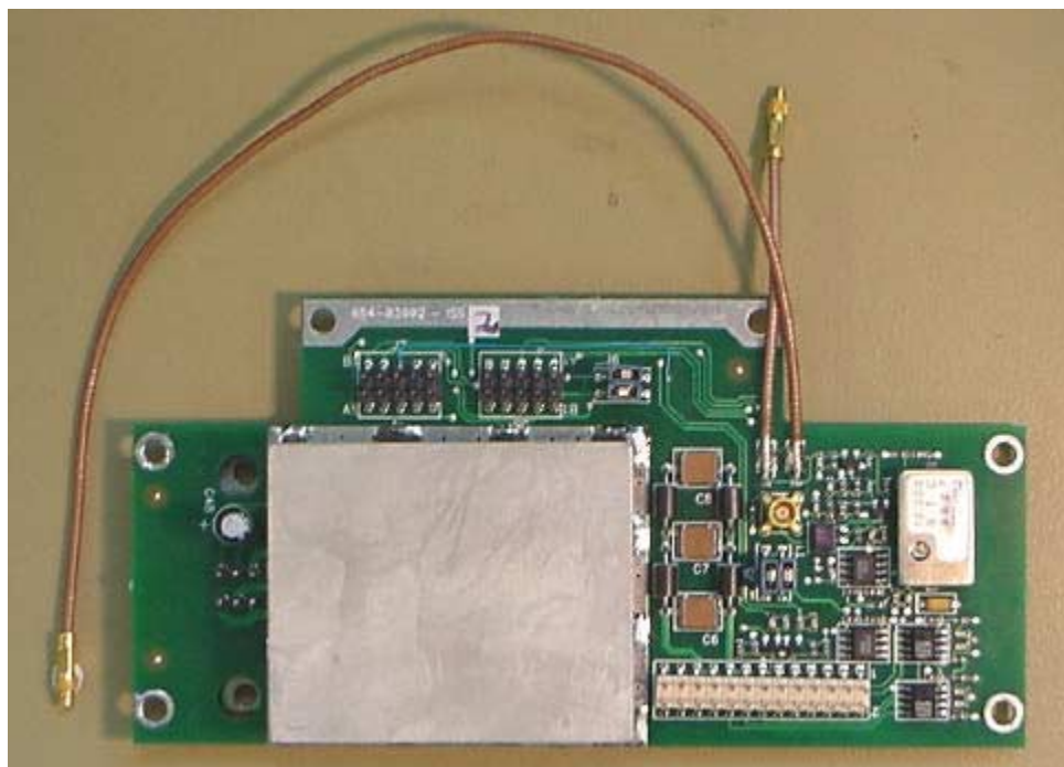
PSU/TCXO PSU Top with Can
