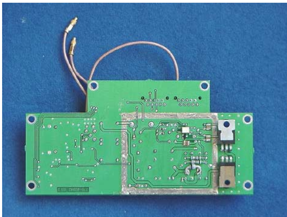
PSU/TCXO PSU Bottom without Can
