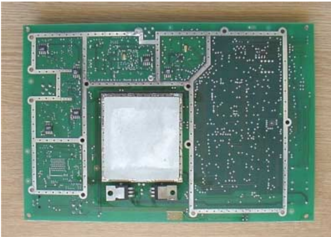
Baseband Processor PCB Bottom with can
