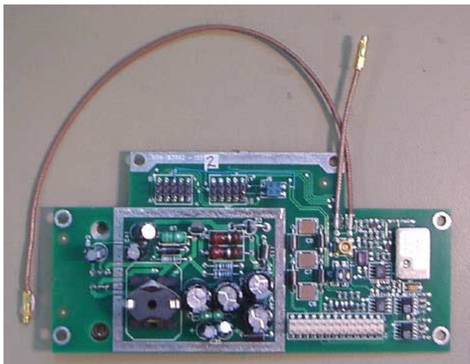
PSU/TCXO PSU Top without Can
