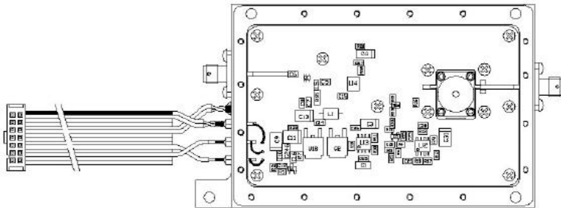
Power Amplifier Open
