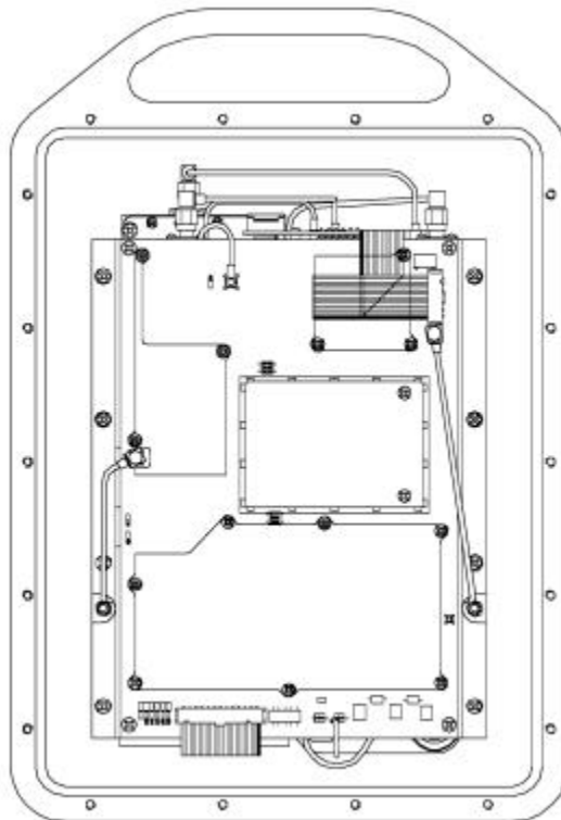
Outdoor Unit without Front Cover
