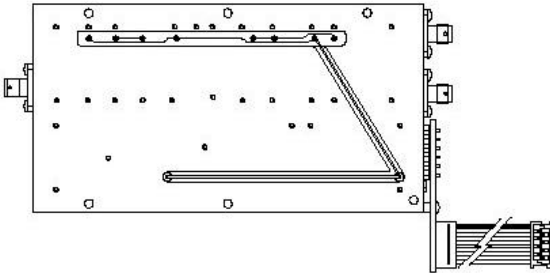
Rx Housing Assembly Bottom
