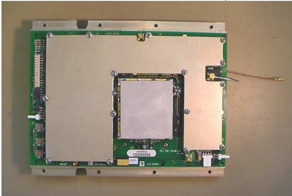
Outdoor Unit with no Baseband Processor Assembly
