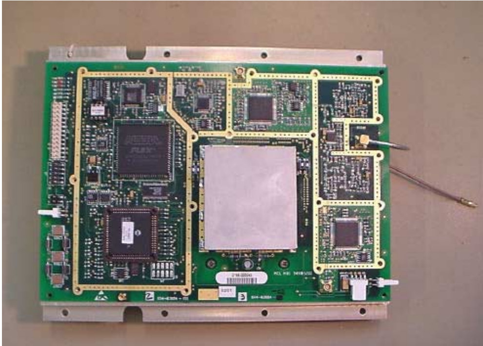
Baseband Processor PCB Top without Cans
