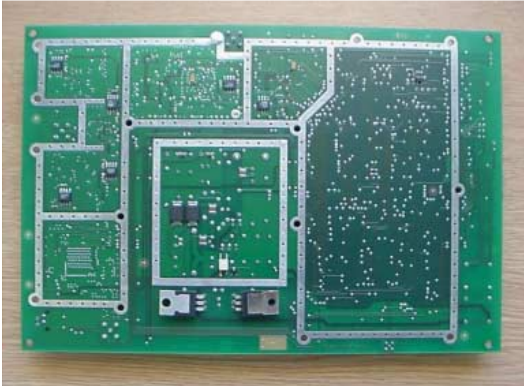
Baseband Processor PCB Bottom without can
