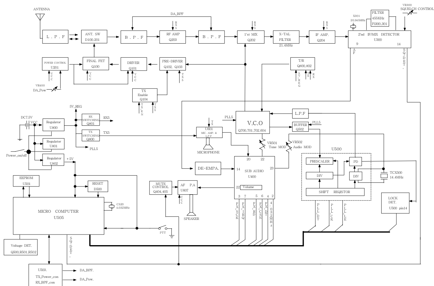
AQ-10 Block Diagram
