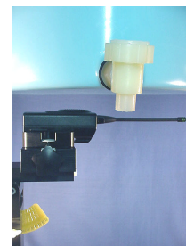
Face-held SAR Test Setup 2.5cm Separation Distance
