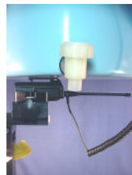
Body-worn SAR Test Setup with 1.0cm Belt-Clip
