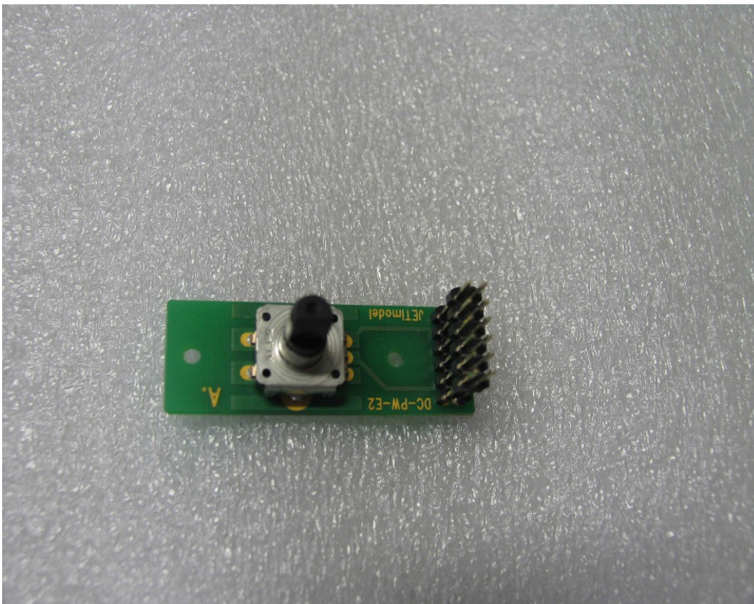
Figure 12 - DS-PW-E2 Board Front
