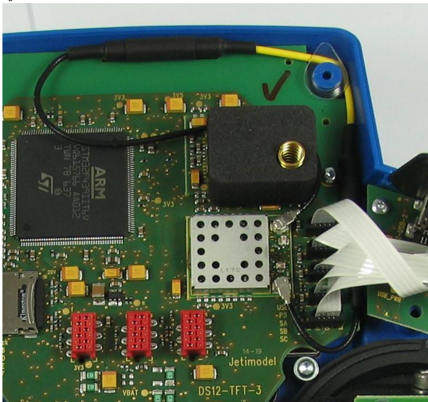
Figure 2a – Antennas 2400MHz
