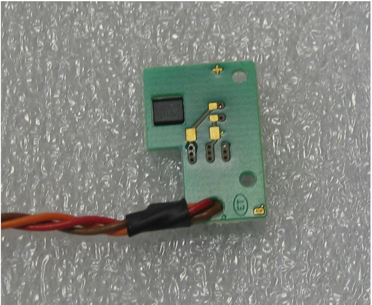
Figure 10: DS-XHall-1 Board Bottom
