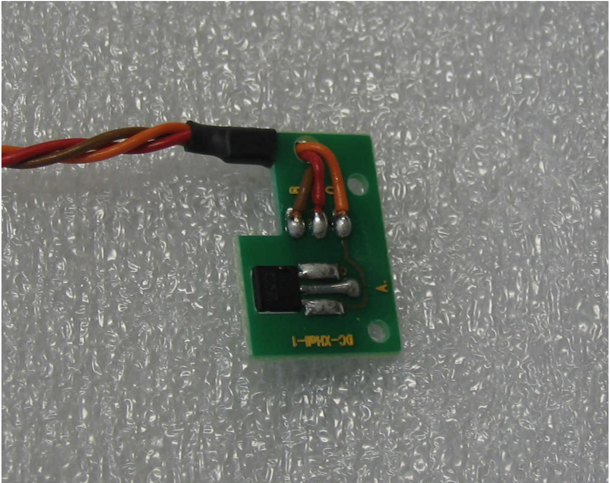
Figure 9: DS-XHall-1 Board Top
