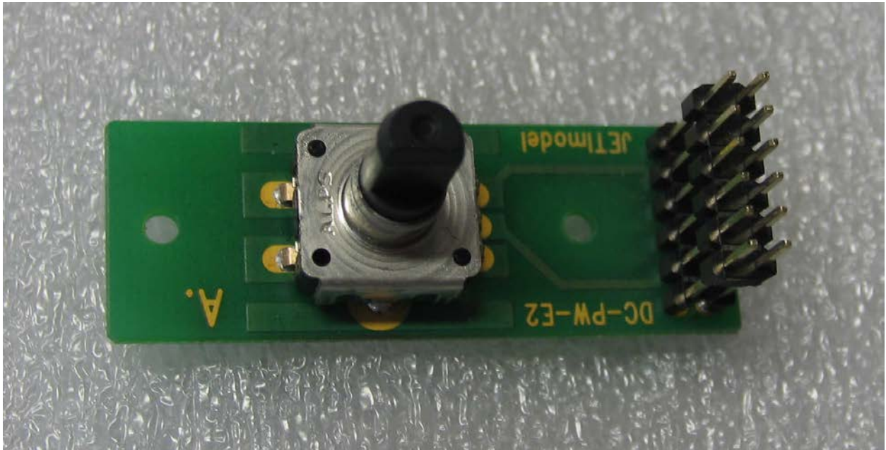
Figure 15: DC-PW-E2 Board Top
