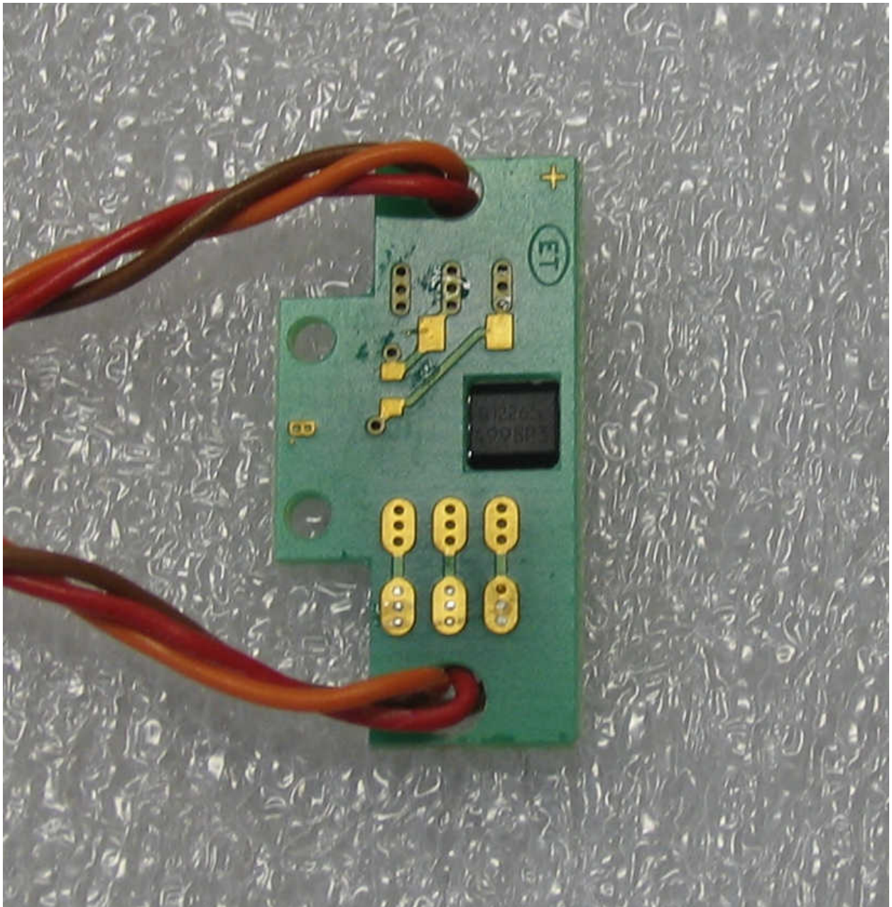
Figure 12: DS-YHall-2 Board Bottom
