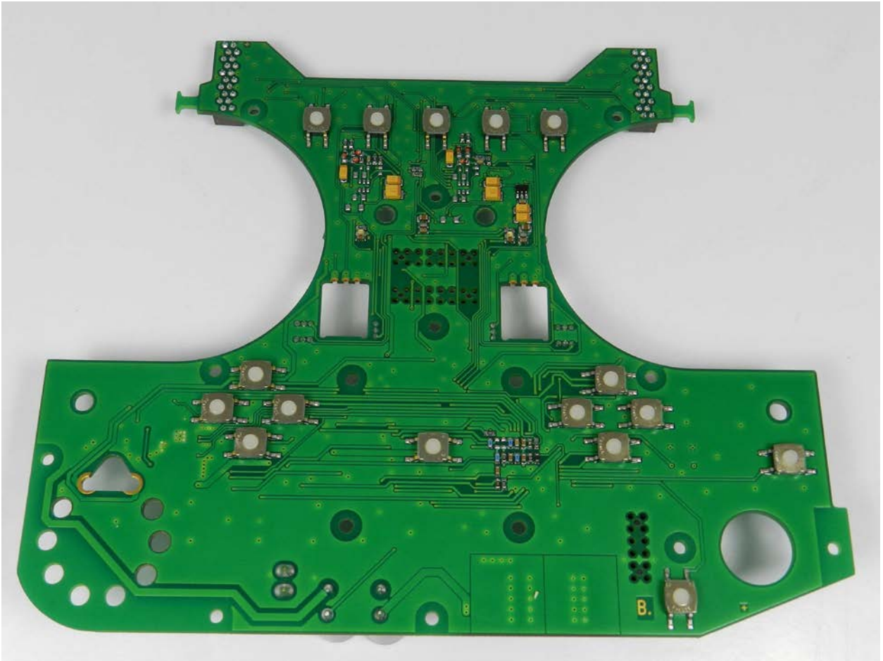
Figure 6: DS-PW-2 Board Bottom
