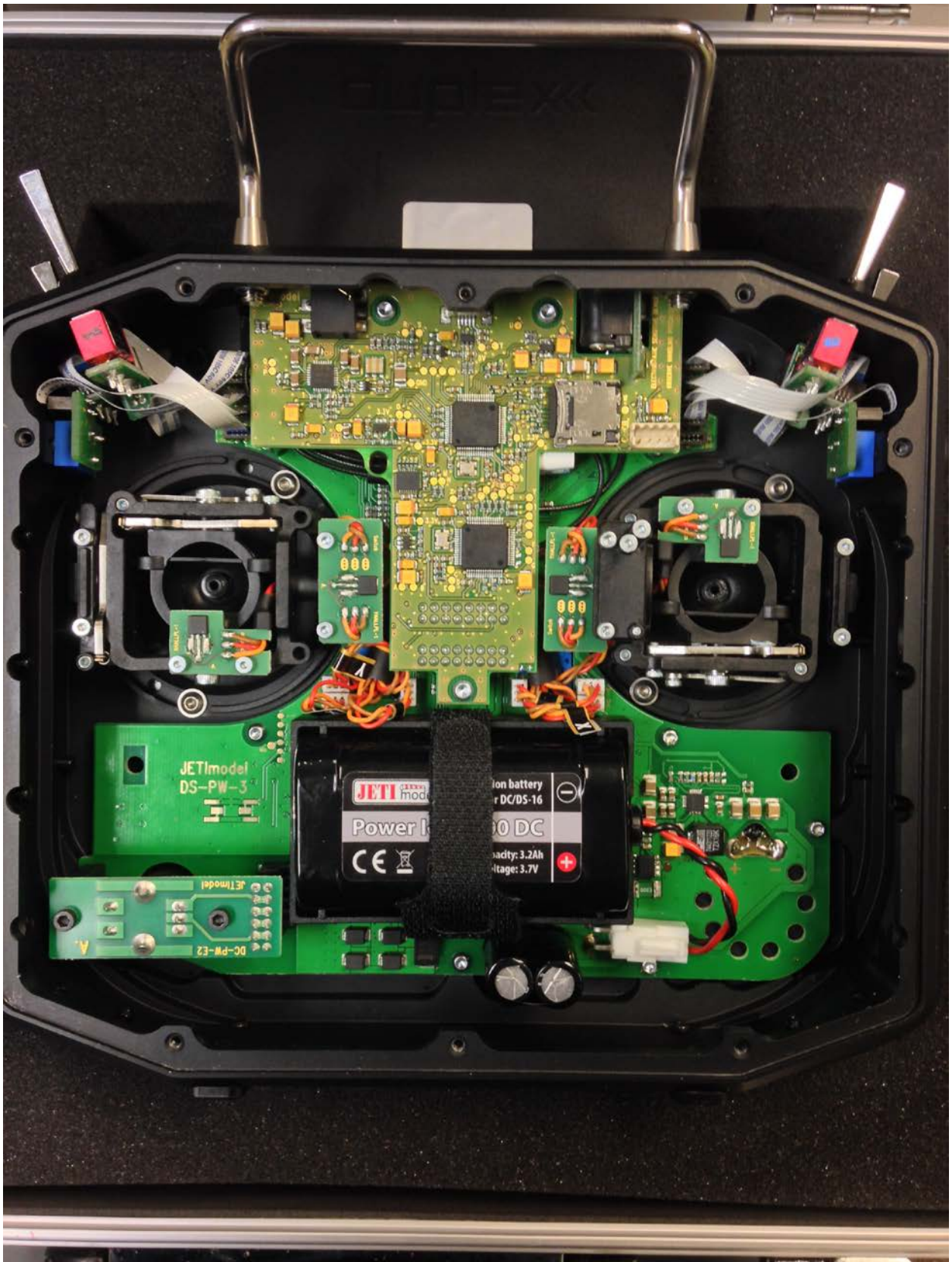
Figure 1: Internal View with back case removed
