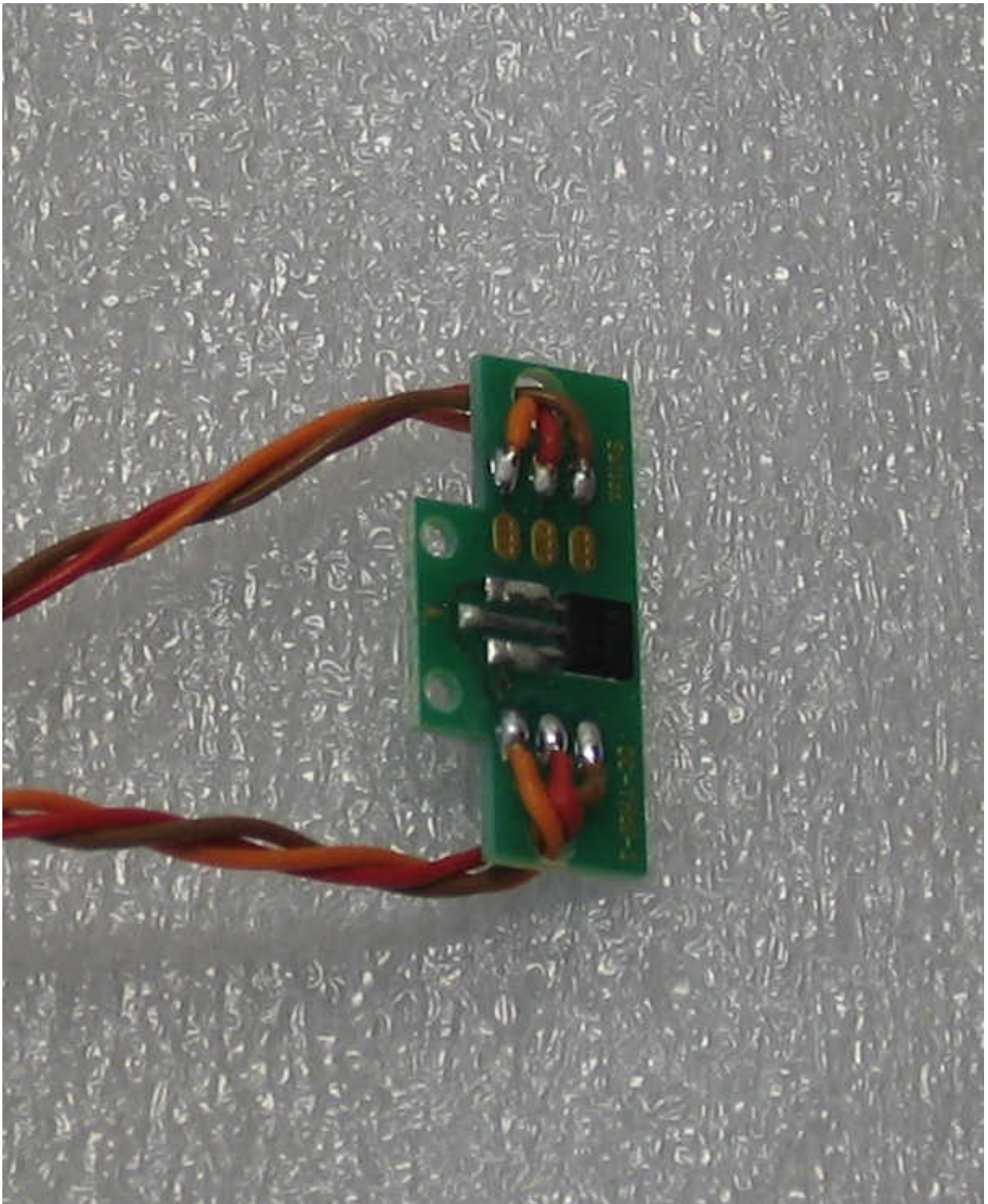
Figure 11: DS-YHall-2 Board Top
