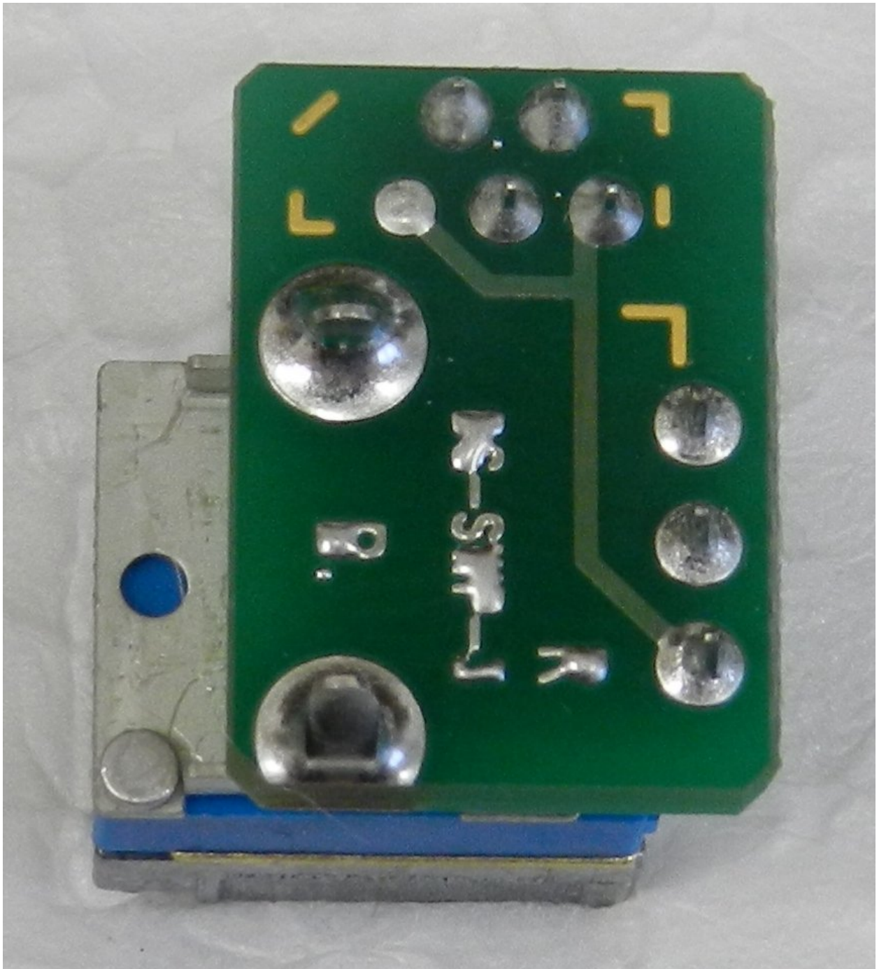
Figure 14: DS-SWP-2 Board Bottom
