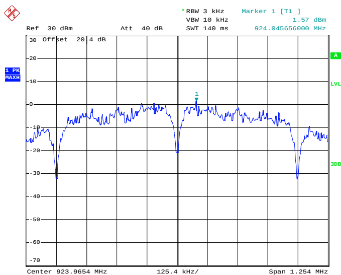
Figure 7.5.2-2: Power Spectral Density - Middle Channel
