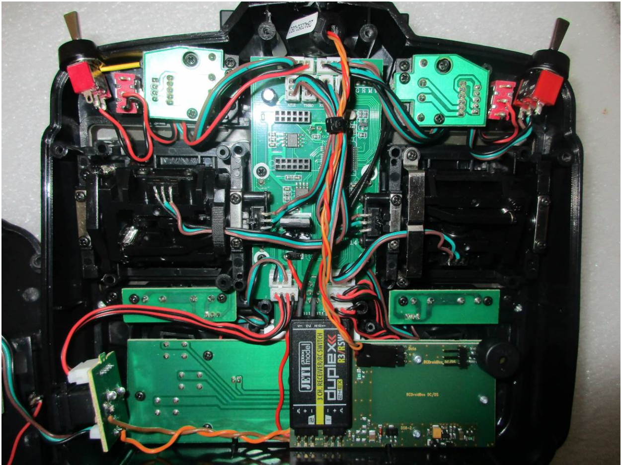
Figure 7: EUT installed in Host – Internal View
