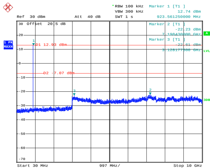
Figure 7.4.2.2-2: 30 MHz – 10 GHz –Middle Channel – Antenna 1
