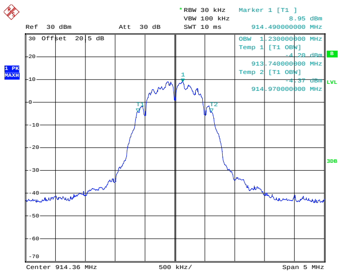
Figure 7.2.2-10: 99% OBW - Low Channel – Antenna 2
