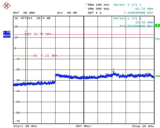
Figure 7.4.2.2-4: 30 MHz – 10 GHz – Low Channel – Antenna 2
