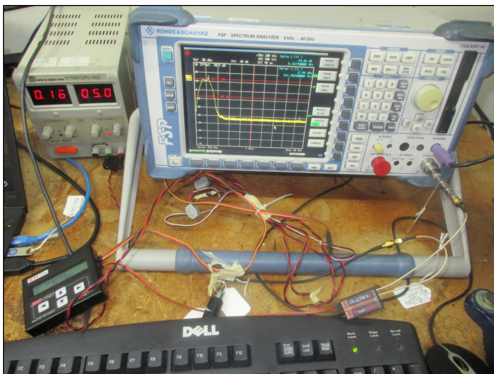
Figure 6: RF Conducted
