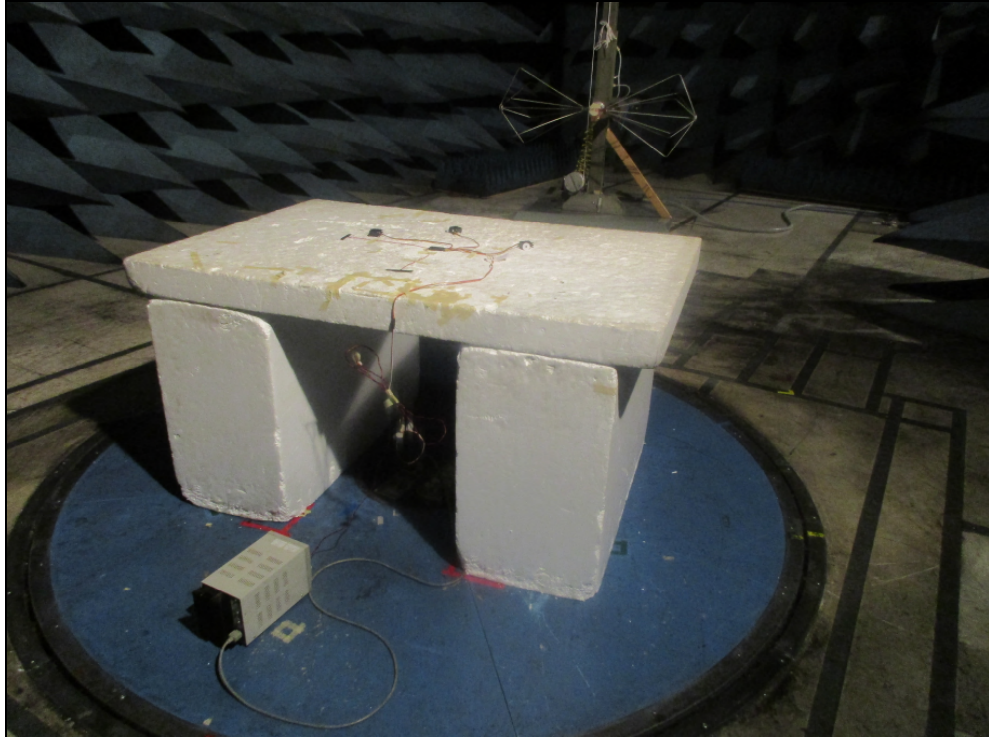
Figure 4: Radiated Emissions – Rear View
