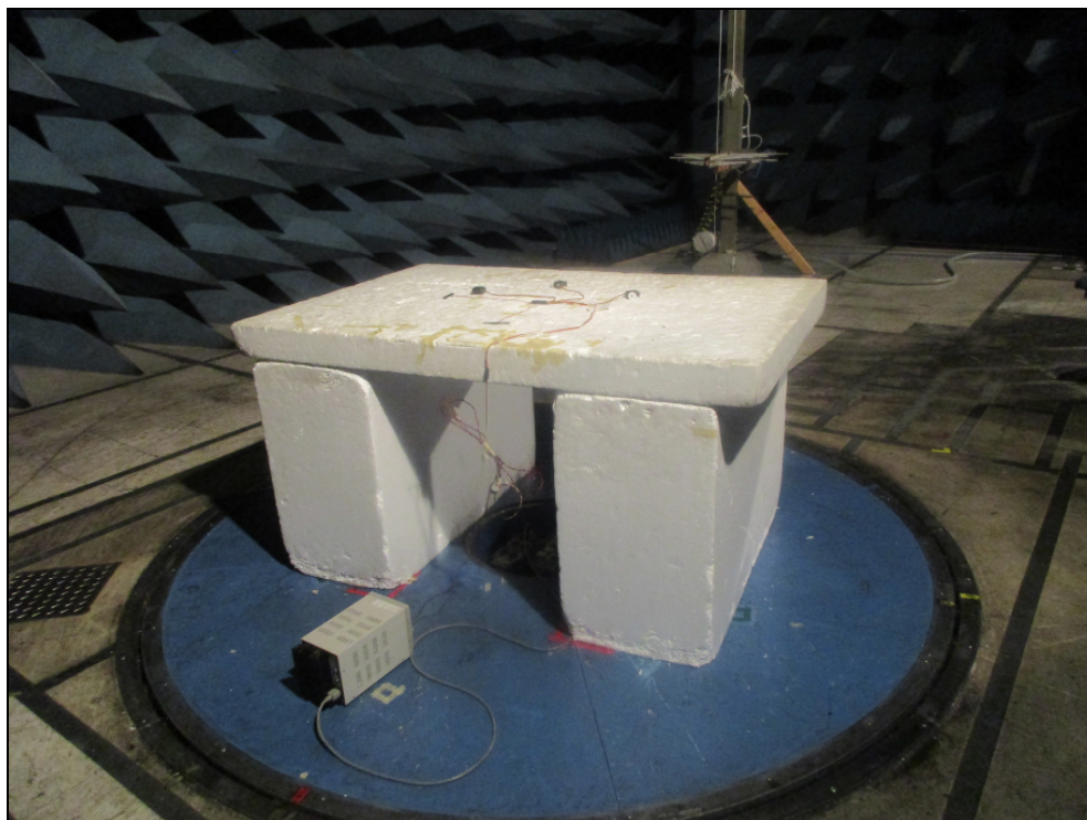
Figure 5: Radiated Emissions – Rear View
