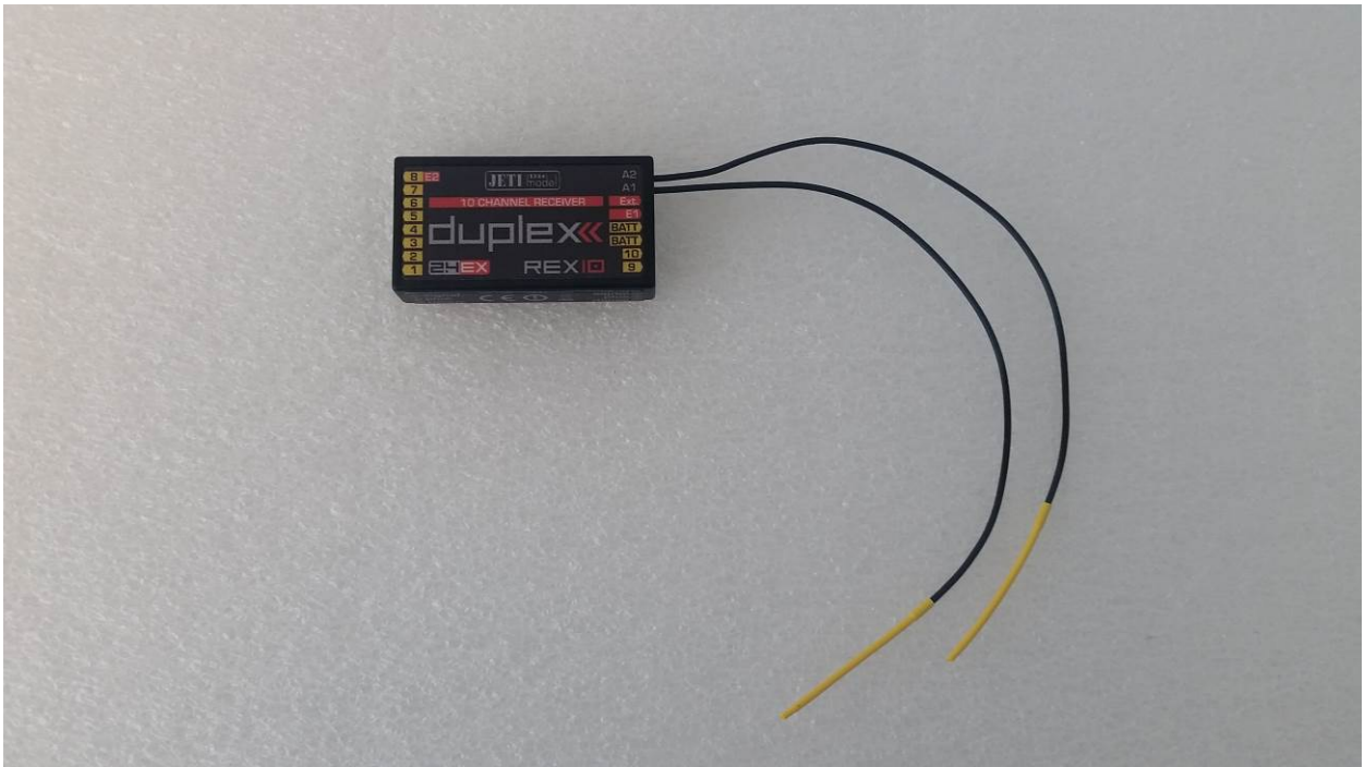
Figure 7: JETIREX10US – Top View
