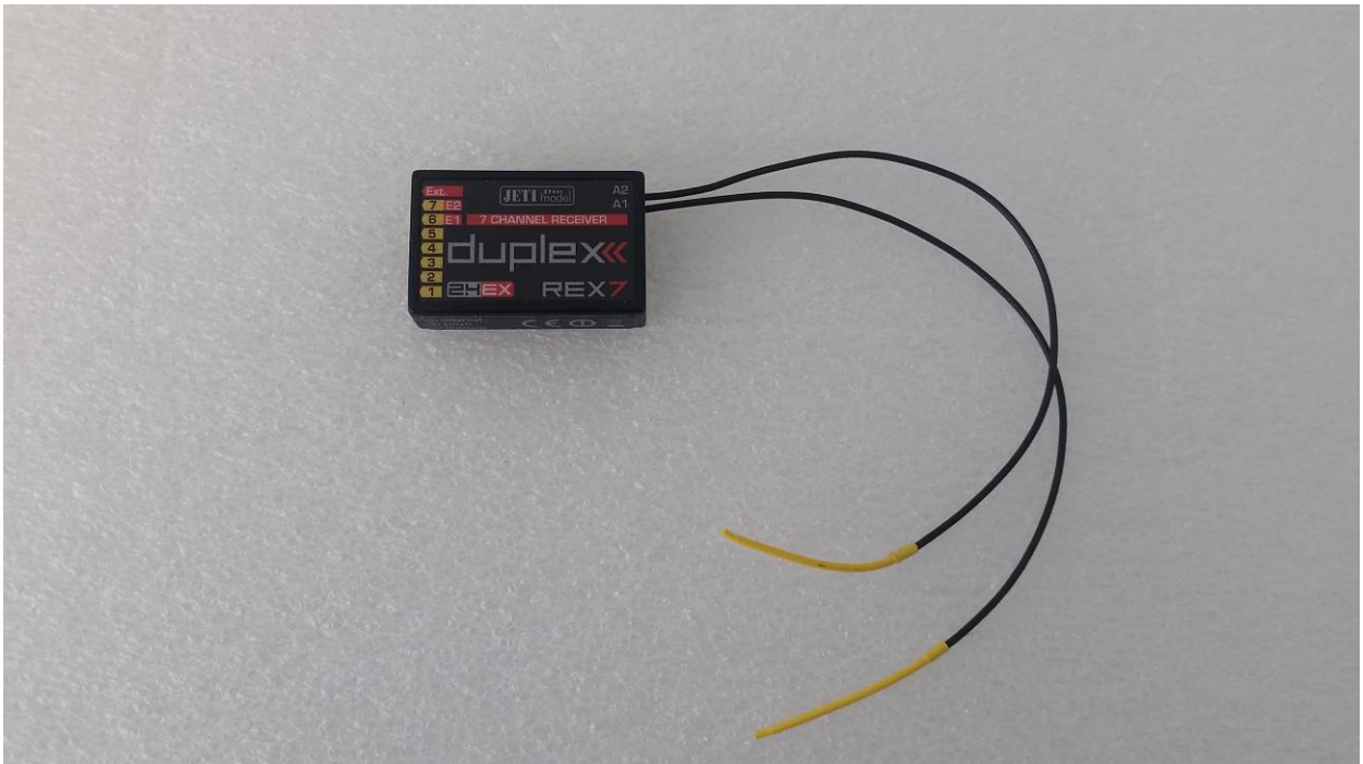
Figure 13: JETIREX7US – Top View
