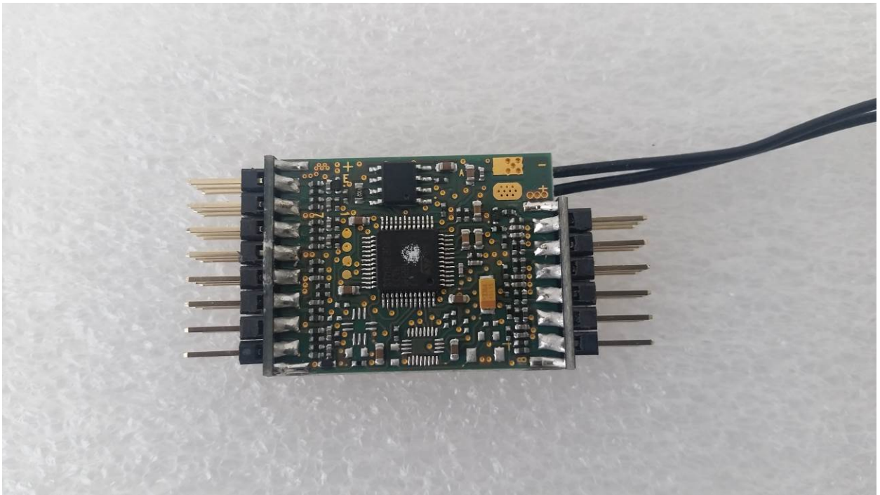
Figure 3: JETIREX10US – Top View
