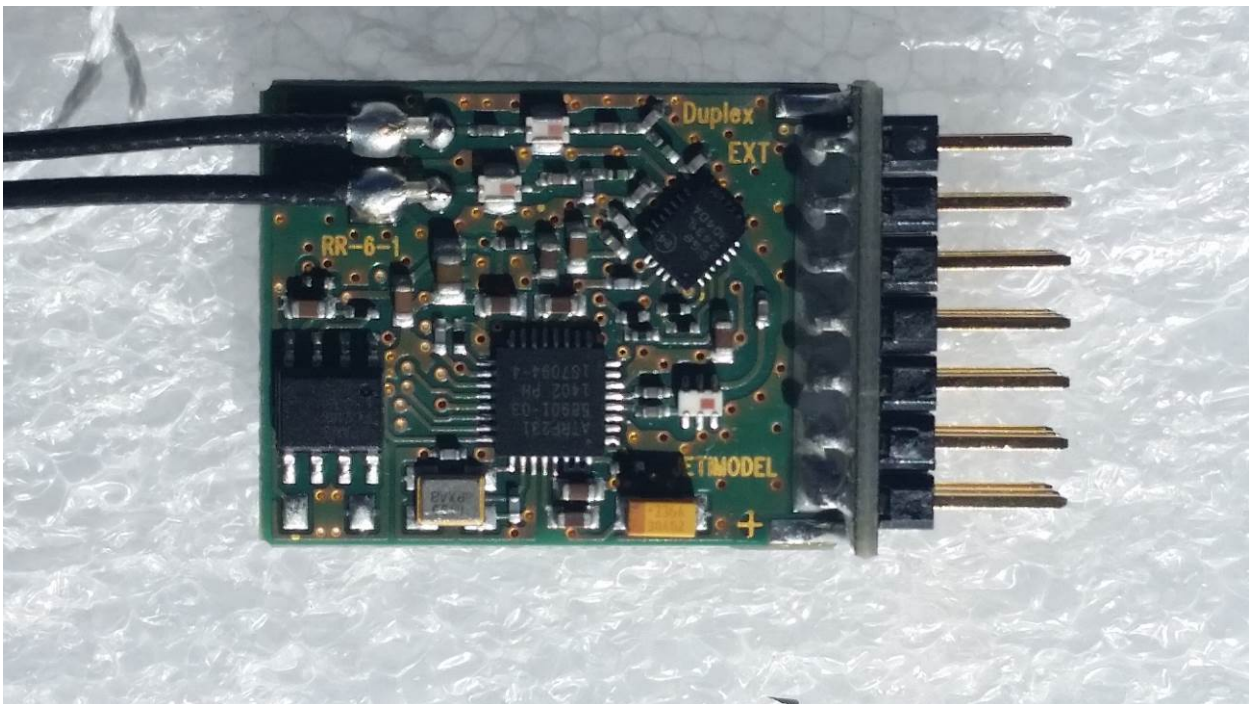
Figure 6: JETIREX7US – Bottom View
