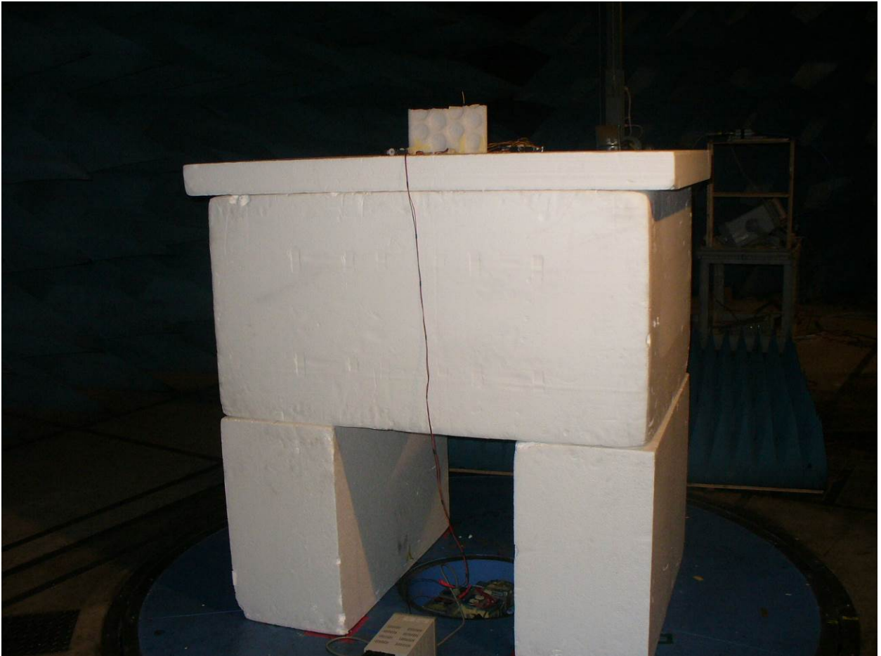
Figure 4: Radiated Emissions – EUT on Side – Rear View
