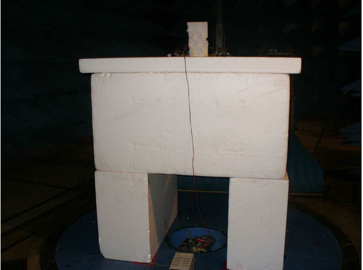
Figure 2: Radiated Emissions – EUT Upright – Rear View
