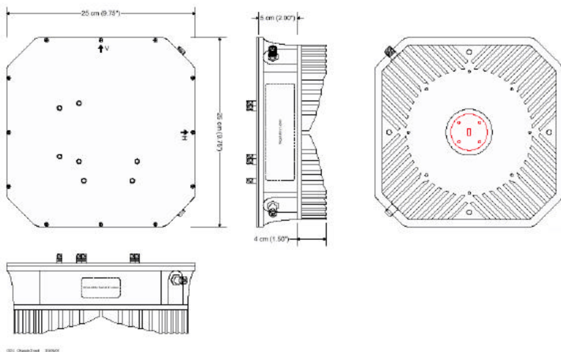
CPE-ODU Elevations with Label Locations
