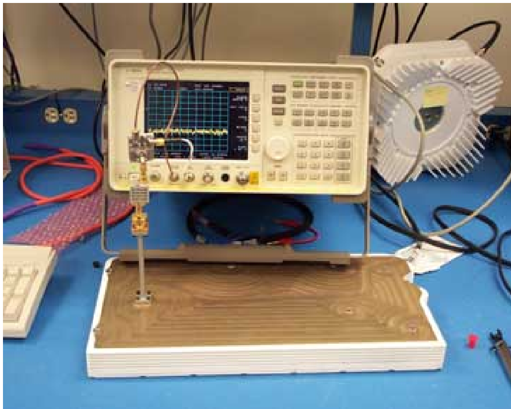
Figure 3 Base Station ODU 40 GHz-200 GHz Test Set Up
