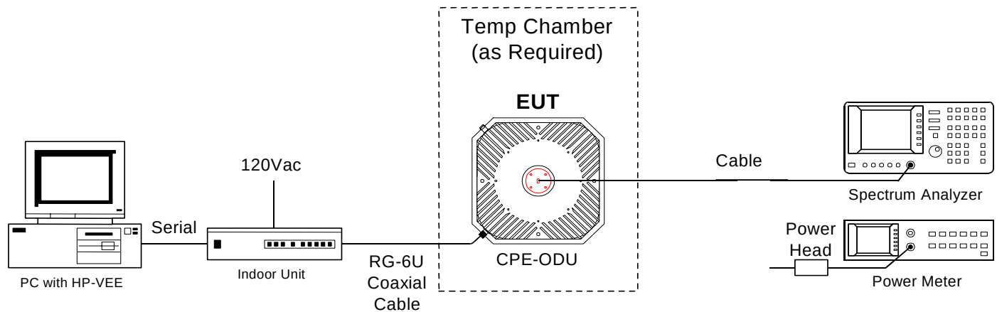
Figure 4 CPE ODU Test Set UP Drawing
