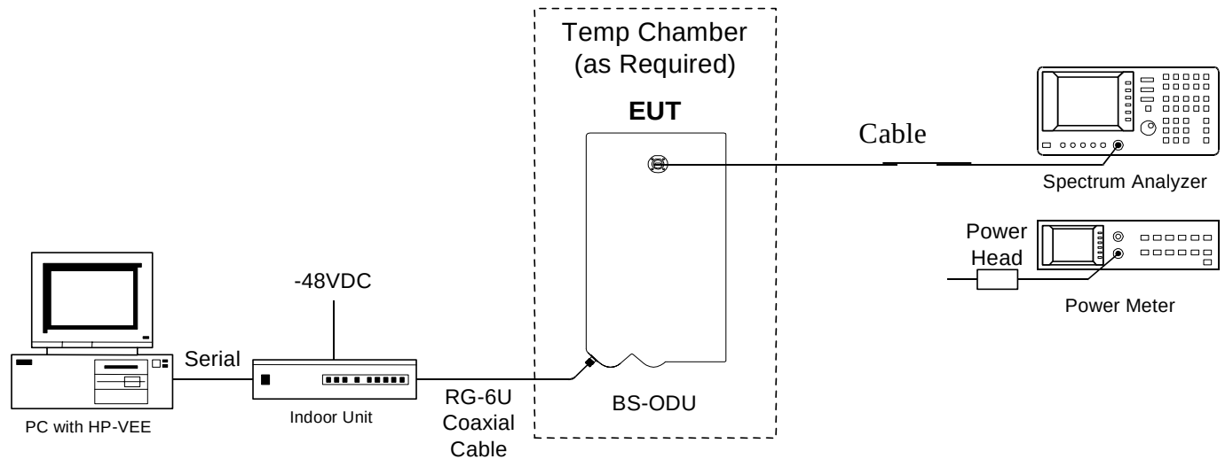
Figure 1 Base Station ODU Test Set Up Drawing
