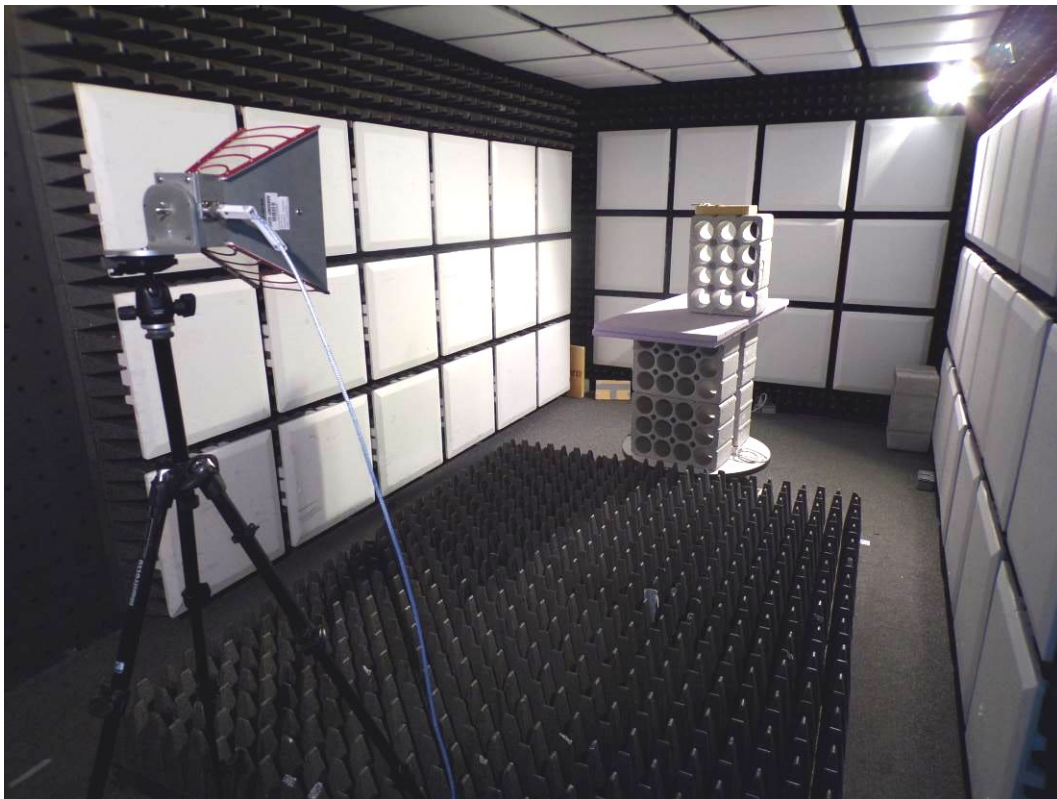
Full Anechoic chamber (Freq > 1GHz)
