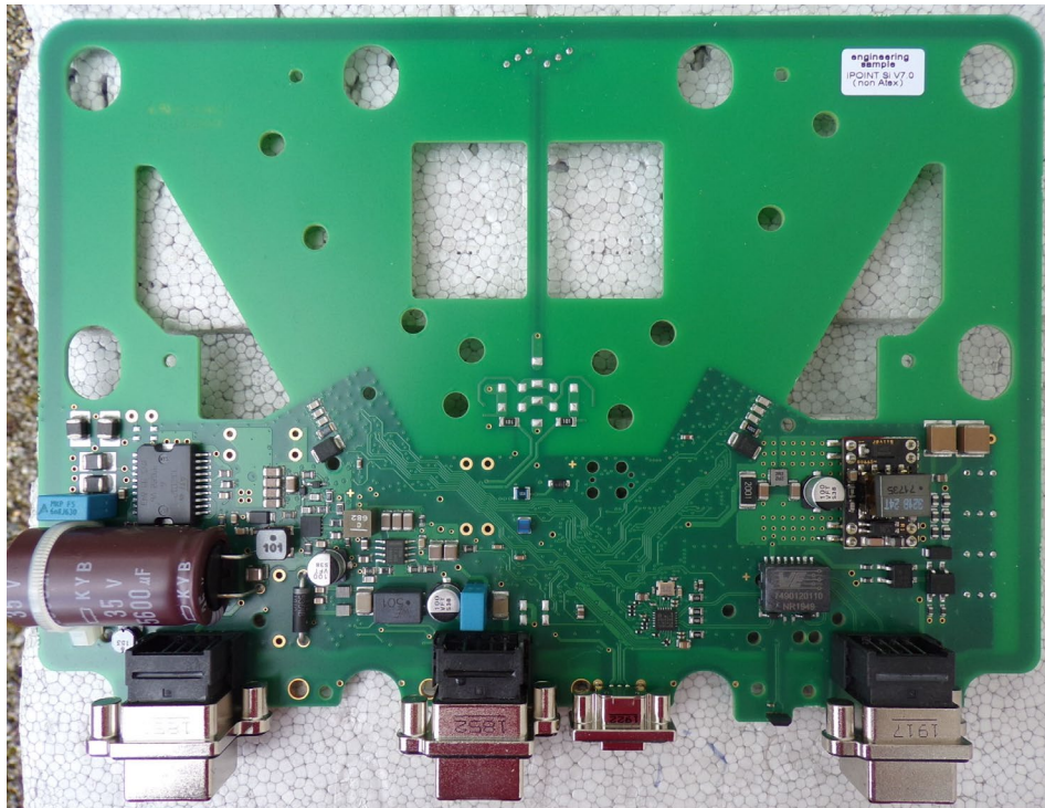
PCB bottom view
