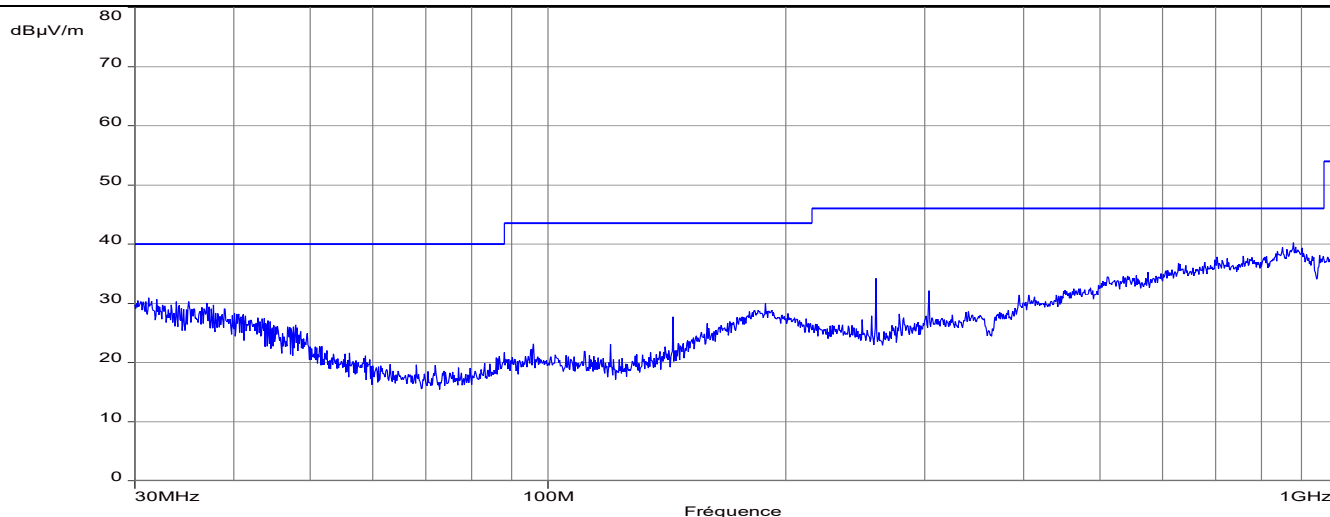
Vertical polarization
