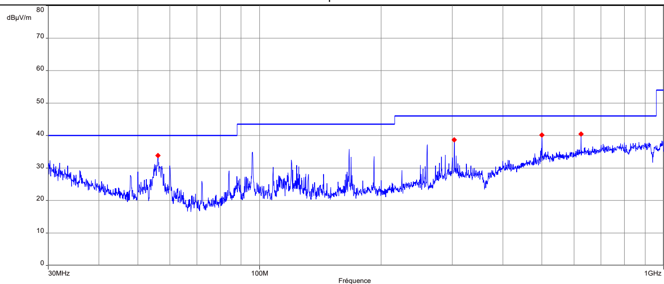
Vertical polarization
