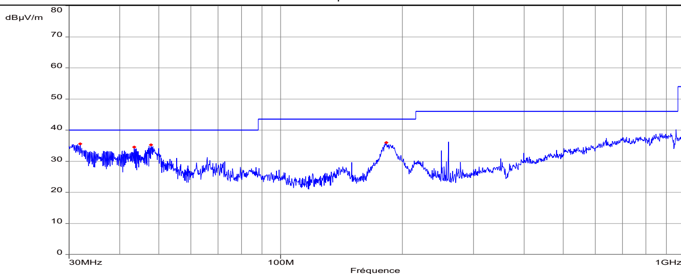
Vertical polarization
