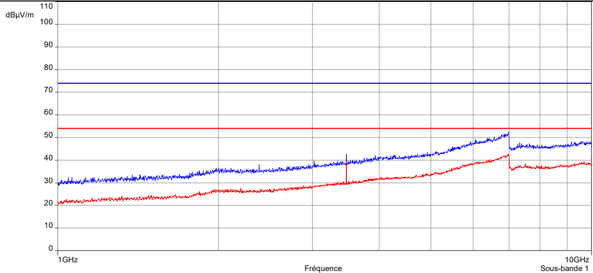
Vertical polarization
