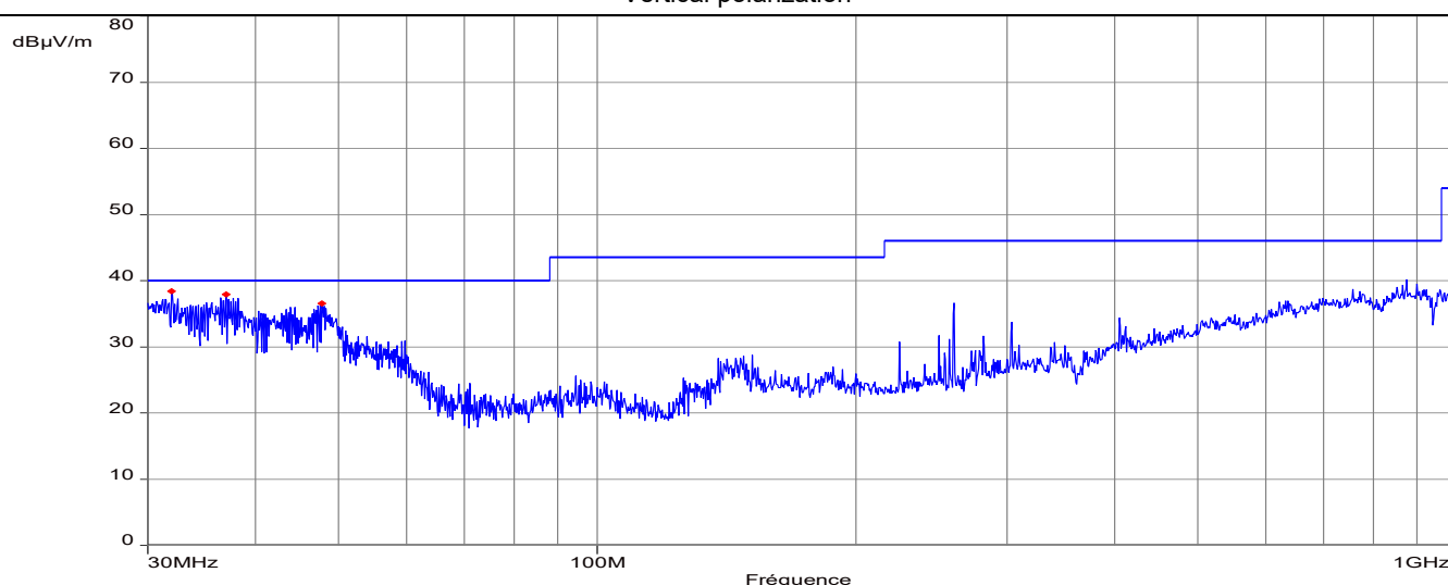
Vertical polarization
