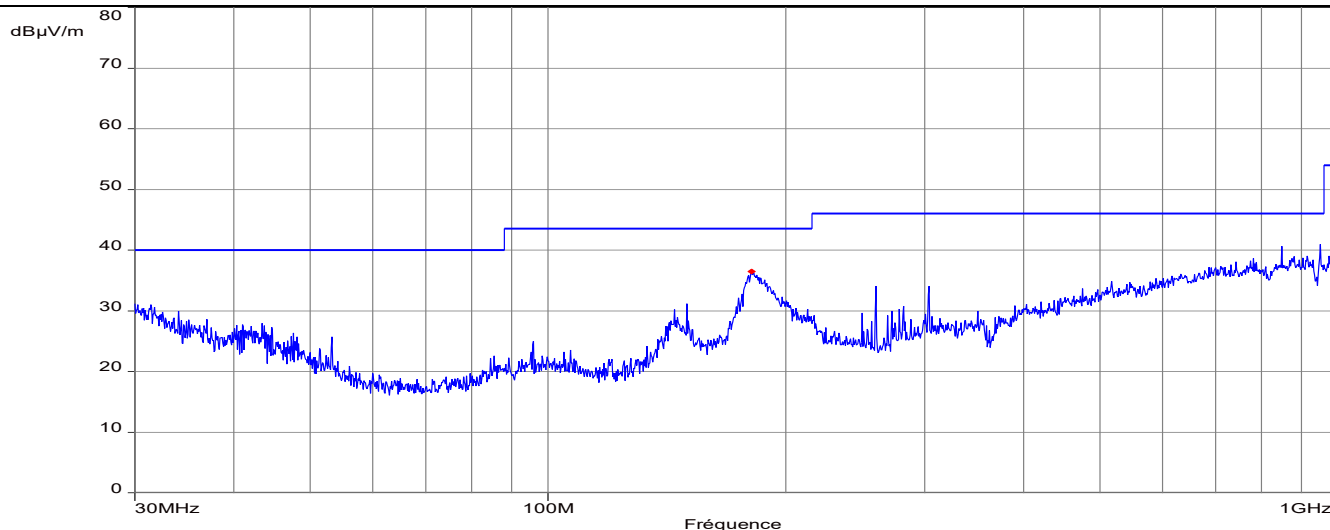
Vertical polarization
