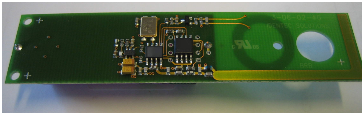
Internal – Bottom View (showing electronics)
