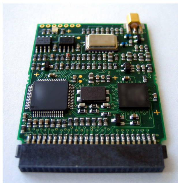
Internal view, CF bus connector
