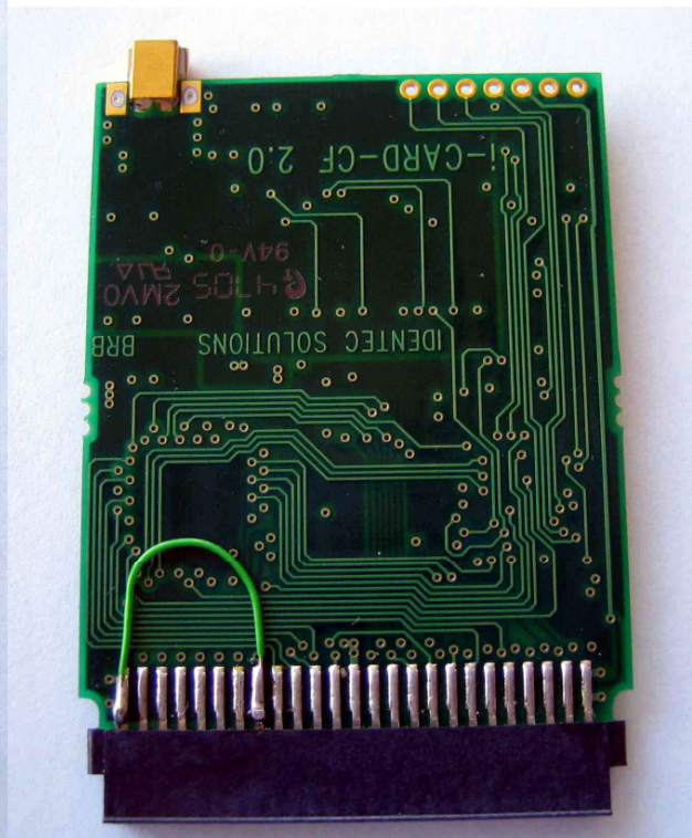
Internal view, rear side
