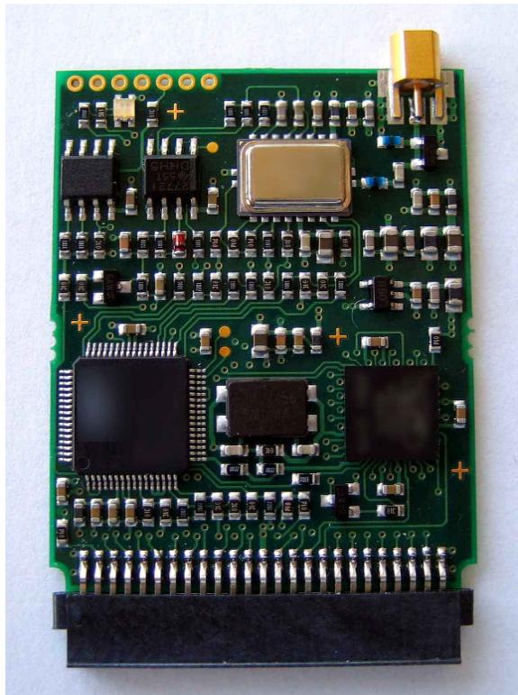
Internal view, front
