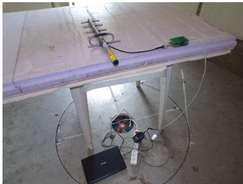
Radiated emission below 1GHz (Antenna type 2-Yagi)
