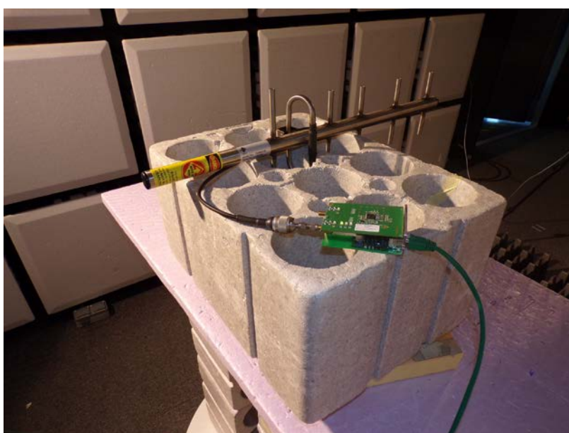
Radiated emission above 1GHz (Anechoic chamber)
