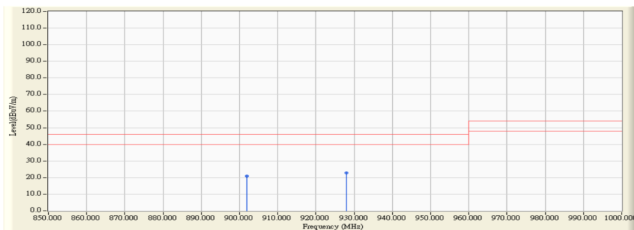
Figure Channel 03: Vertical (Quasi-Peak)
