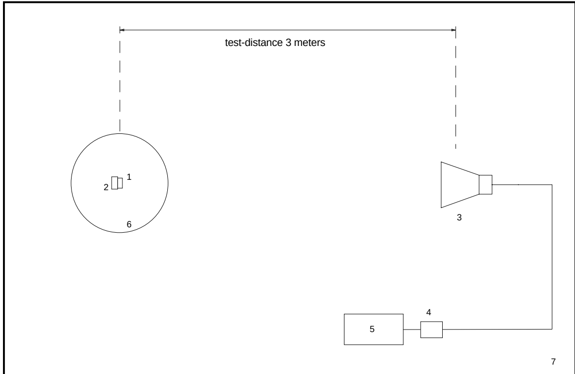
Figure 2: Measurement setup for radiated emission test above 1 GHz
