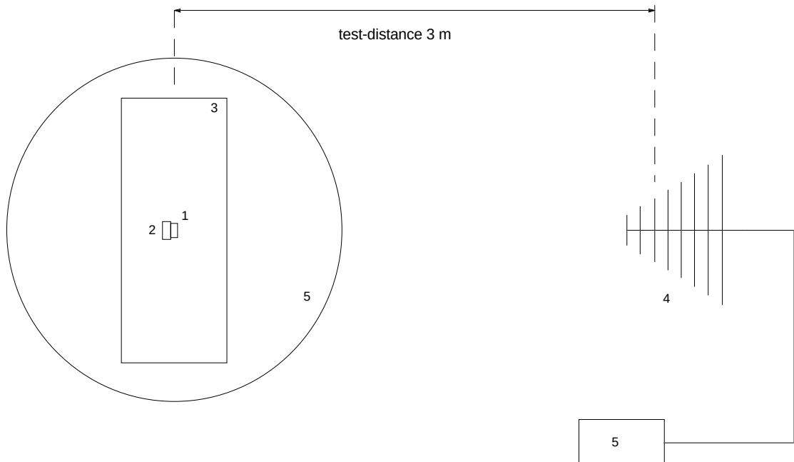
Figure 1: Measurement setup for radiated emission test below 1 GHz
