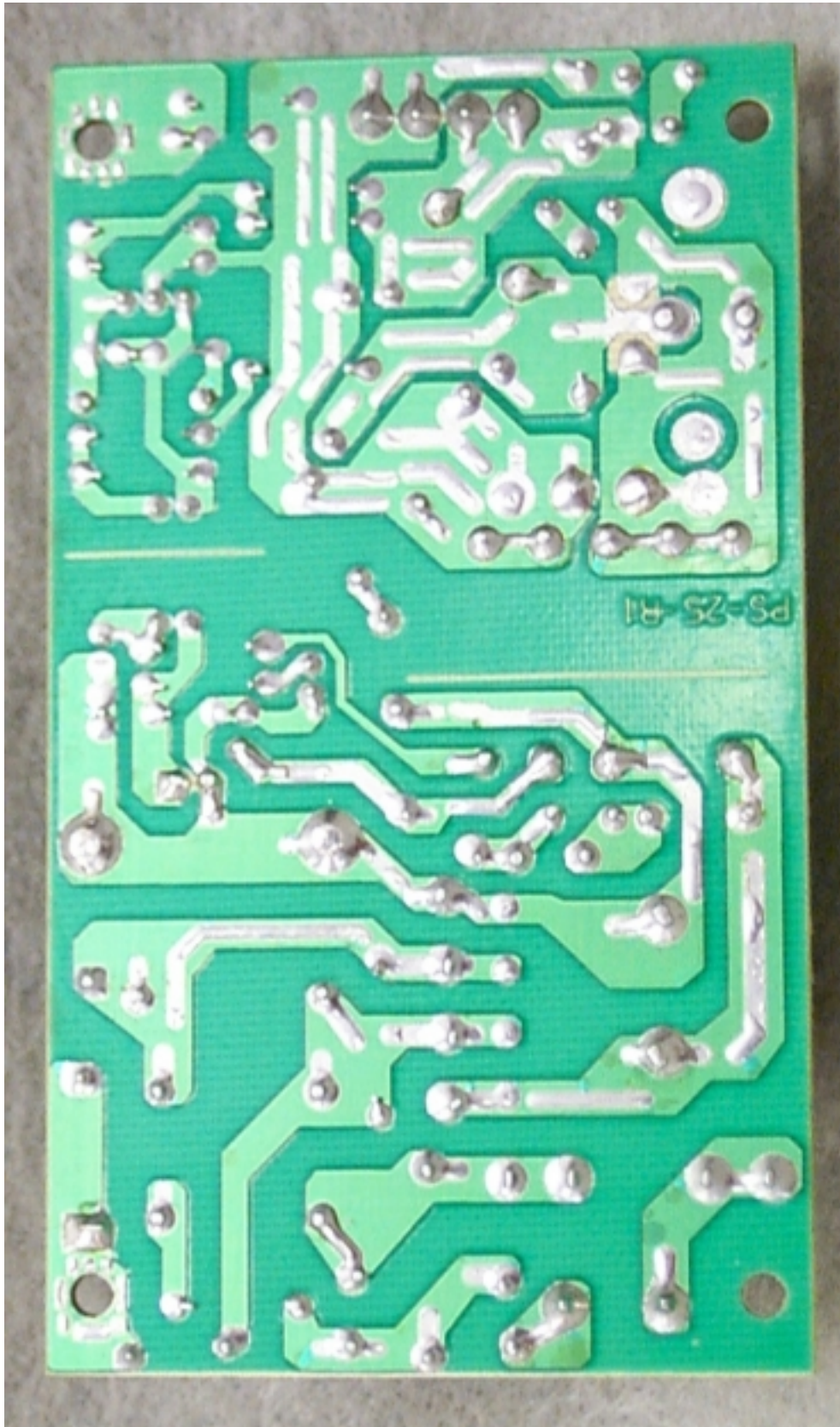
Photo 7. EUT, Bottom View of Power Supply
