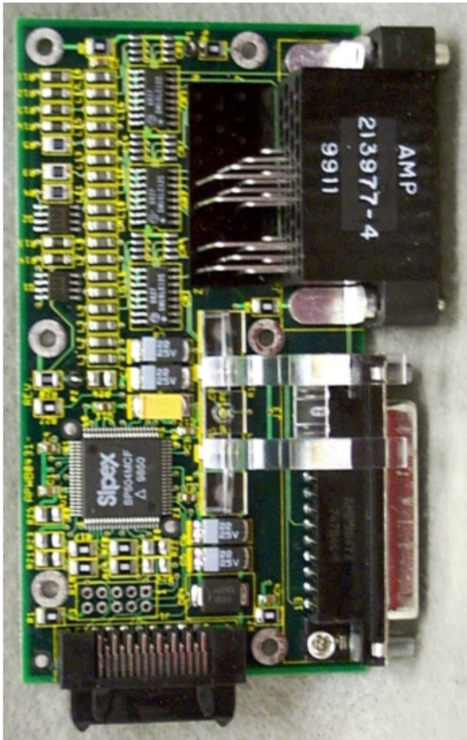
Photo 11. EUT, Top View of SIU Board
