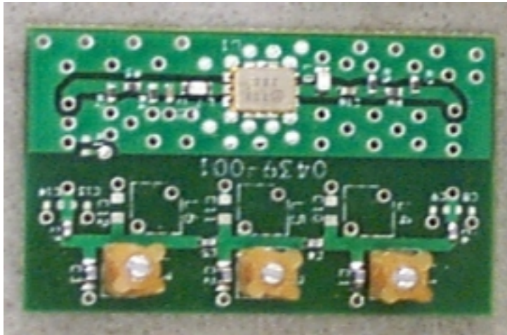
Photo 25. EUT, Top View of 512k IF Filter Board Installed within Transceiver Board
