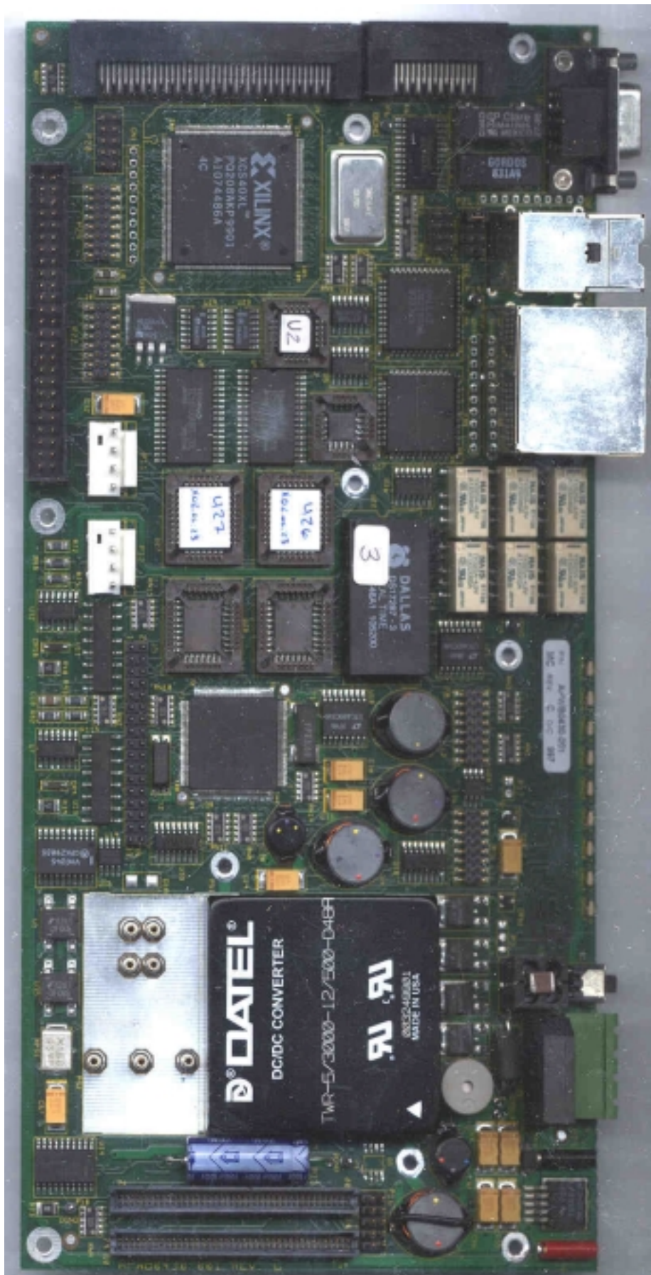
Photo 15. EUT, Top View of CTU Board
