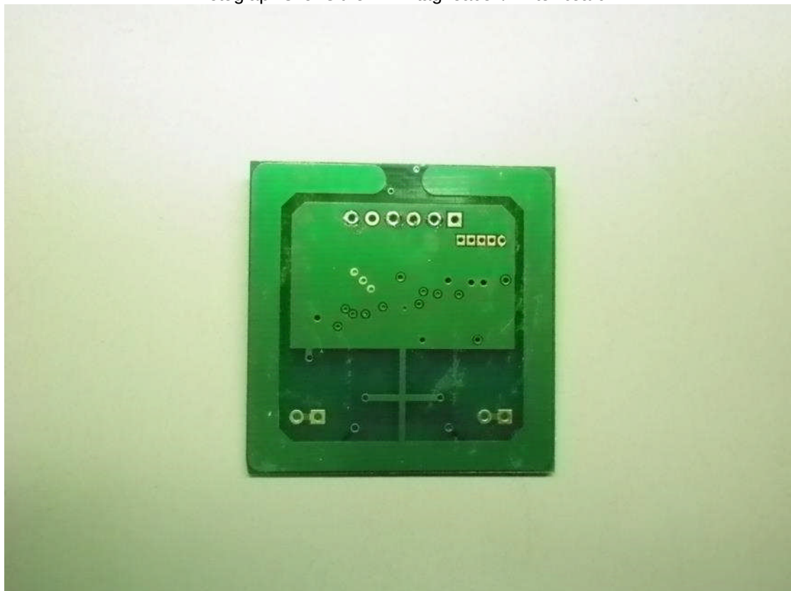
Photograph shows the RFID tag reader / writer board. The antenna element is shown etched into the printed circuit board.
