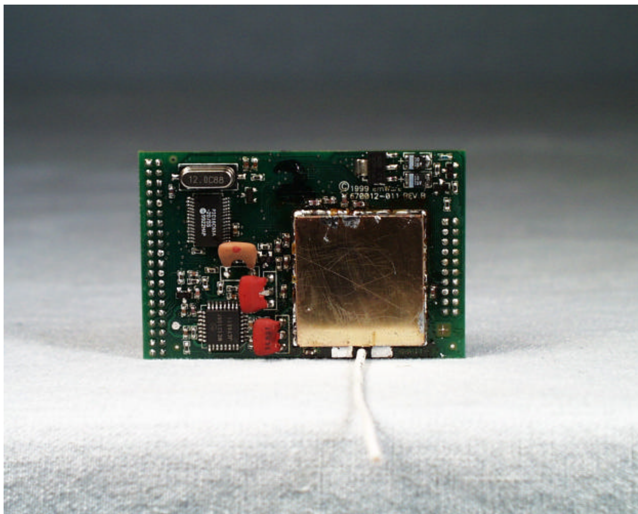
Front view of the EMRF900 with RF cans installed
