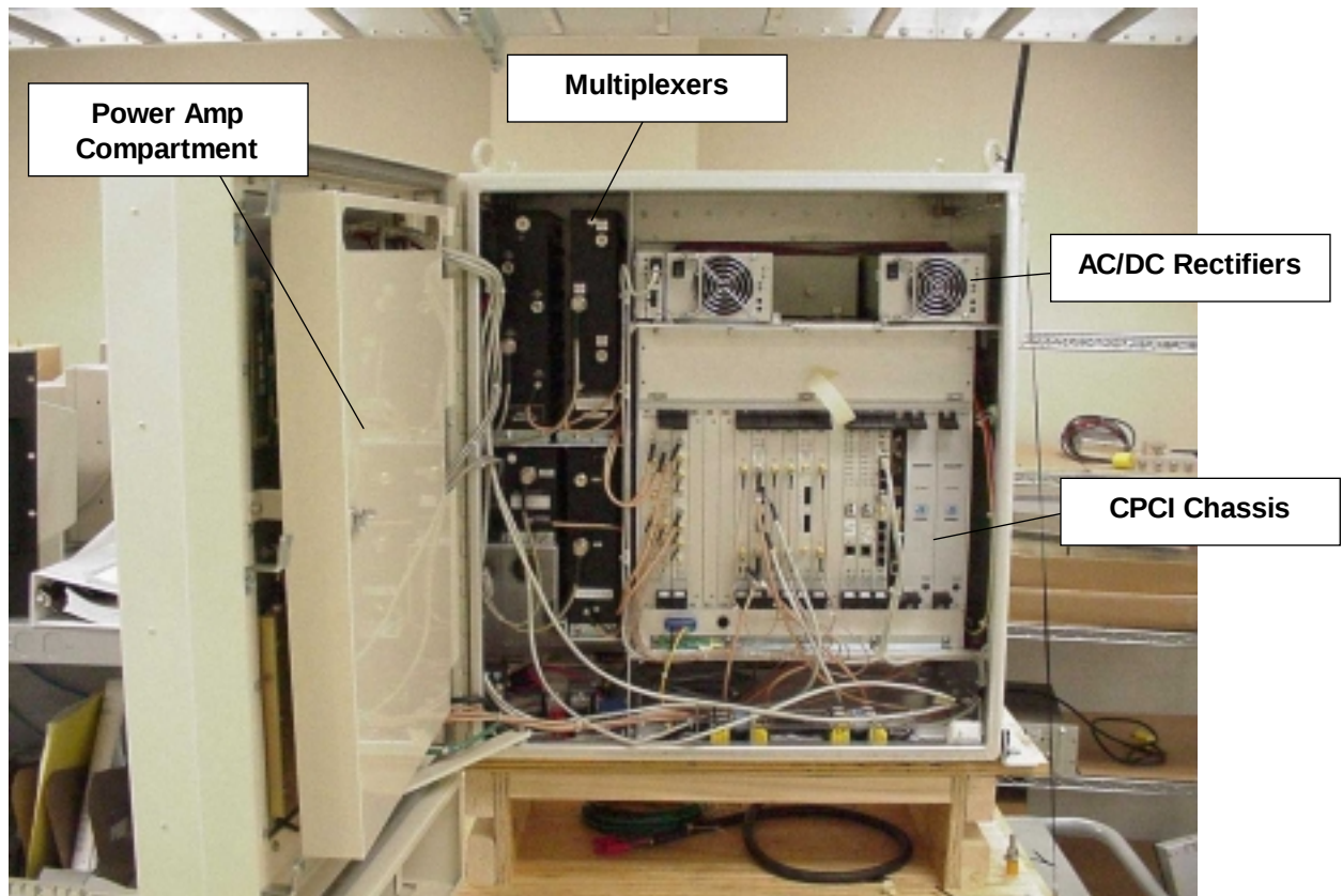
Figure 6-1 RAN, door open
