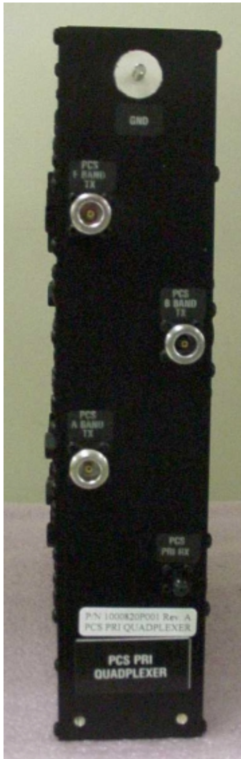
Figure 6-4 Quadplexer, PCS Primary (Transmitting Blocks A/B/F)
