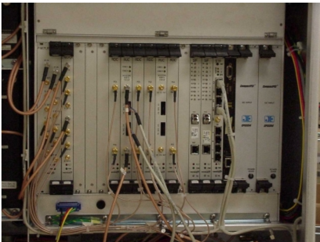
Figure 6-2 RAN Compact PCI chassis
