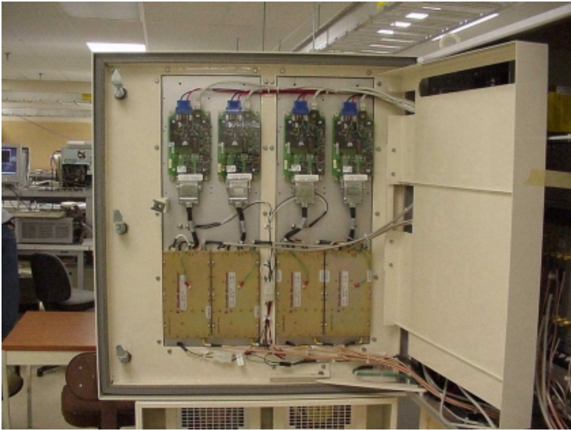
Figure 6-8 Power Amplifiers installed in RAN
