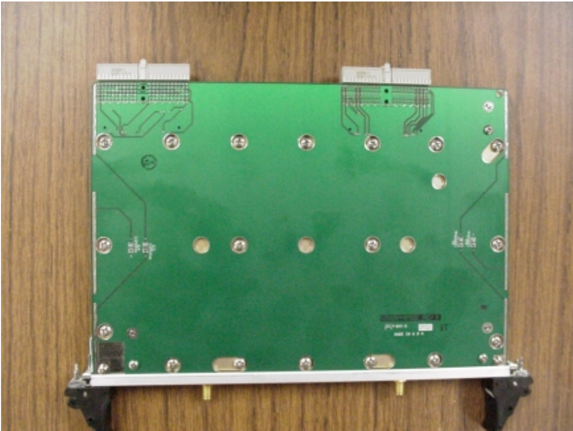
Figure 6-12 RUC Module, Bottom View
