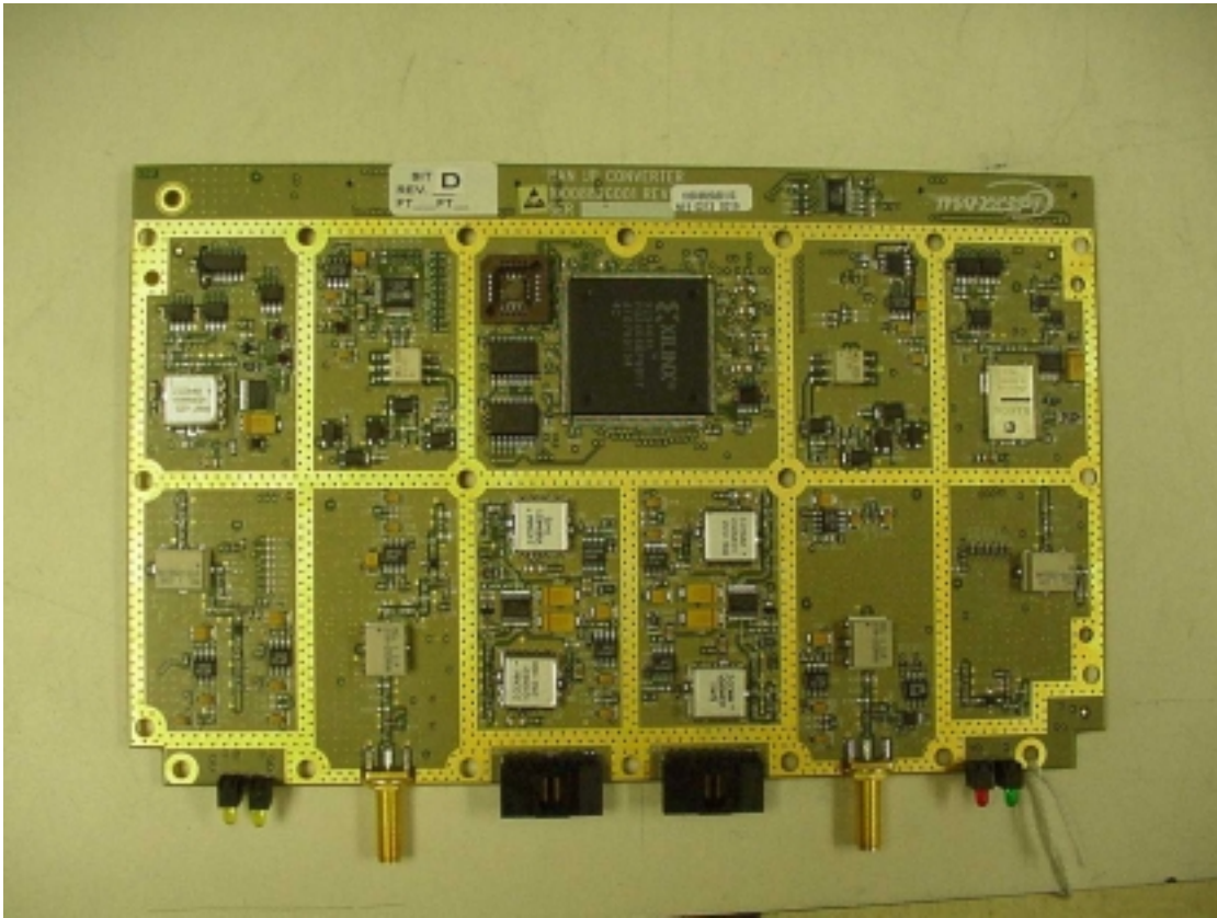
Figure 6-11 RUC circuit card (shield removed)
