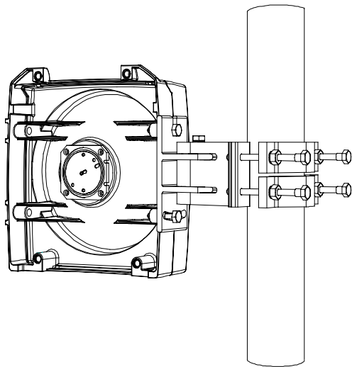
Figure 1.1 Compact antenna.
