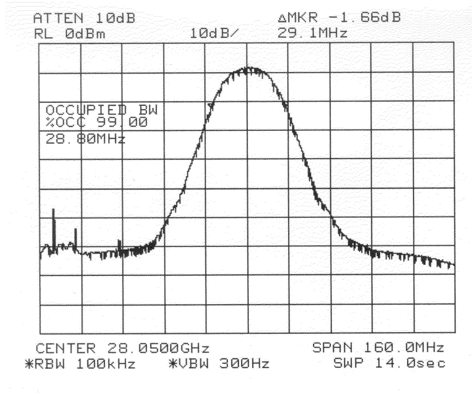
Figure 2- Occupied bandwidth measurement
