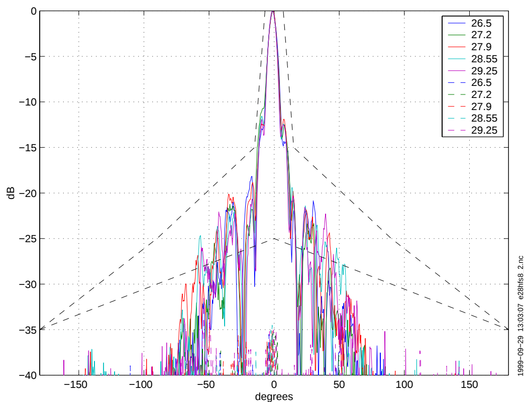
Figure 12 Co- and cross-polar radiation patterns in elevation for antenna 8.
