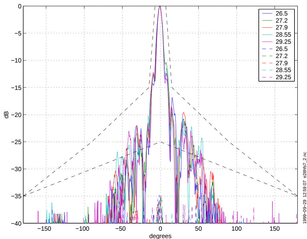
Figure 11 Co- and cross-polar radiation patterns in elevation for antenna 7.
