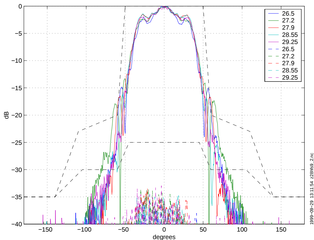
Figure 9 Co- and cross-polar radiation patterns in azimuth for antenna 9.
