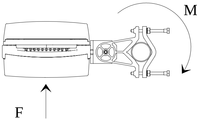
Figure 4.1 Wind load and torque.
