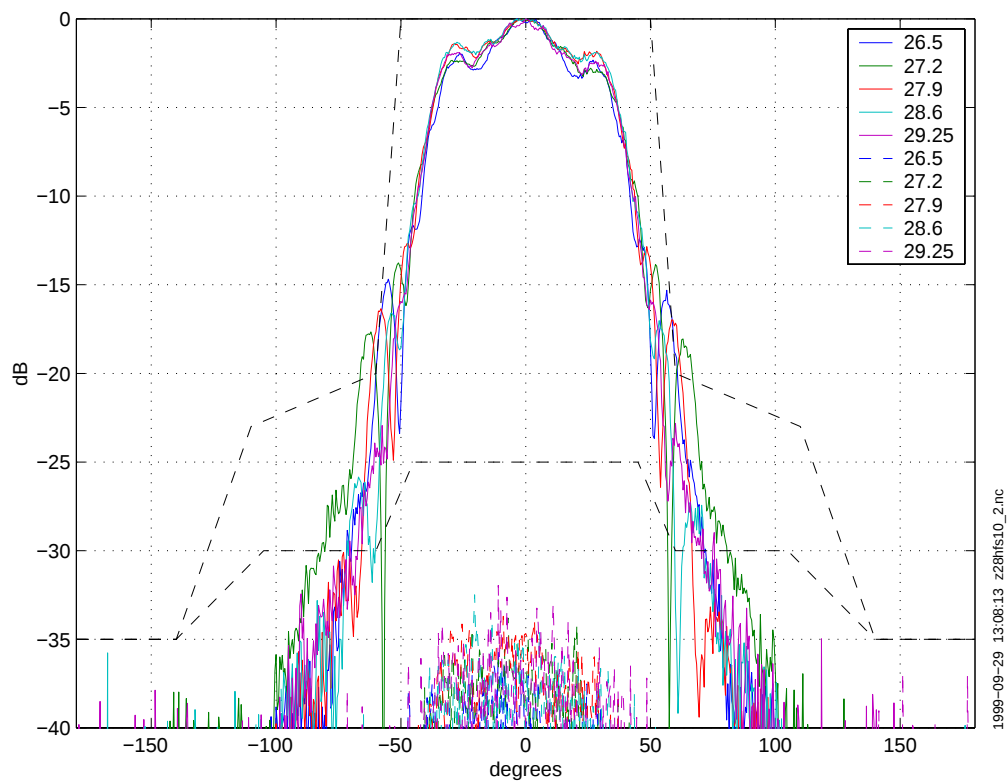
Figure 10 Co- and cross-polar radiation patterns in azimuth for antenna 10.
