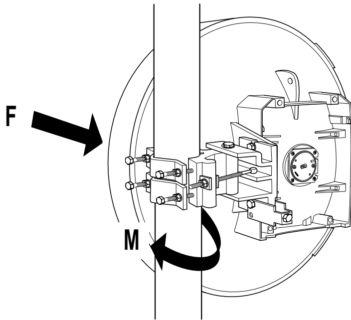
Figure 10-2 Wind Load
