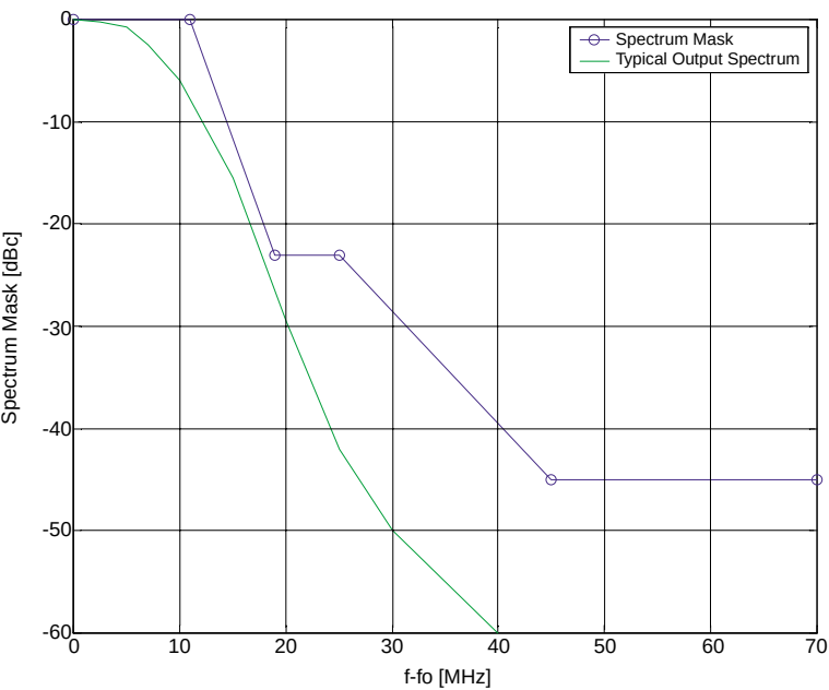
Figure 10–1 Transmitter Mask
