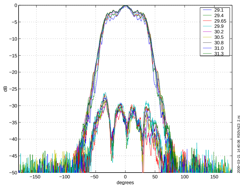
Figure 13 Radiation patterns in azimuth for A23000HUJ9.
