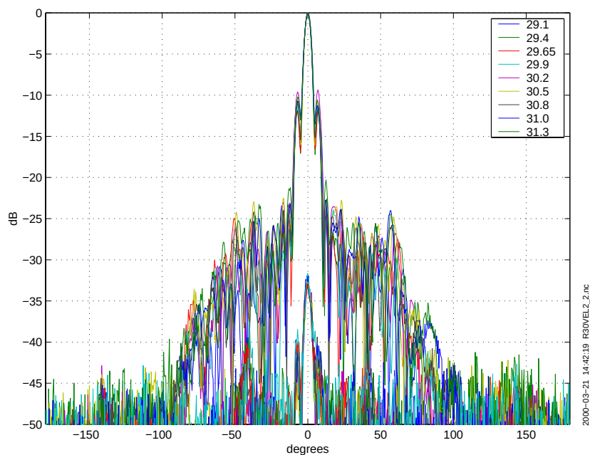
Figure 15 Radiation patterns in elevation for A23000HUJB.
