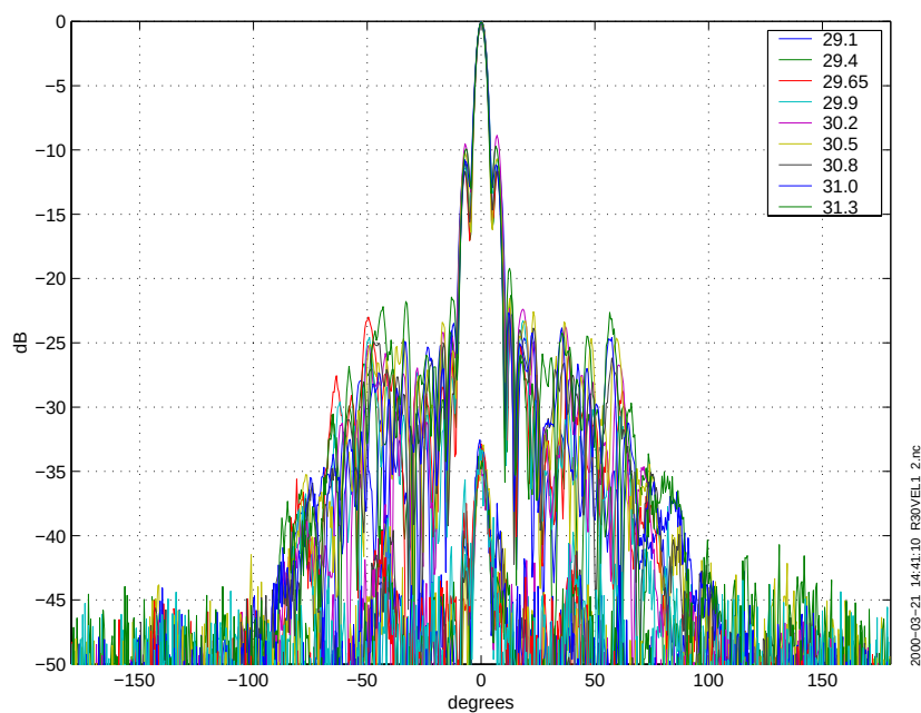
Figure 14 Radiation patterns in elevation for A23000HUJA.
