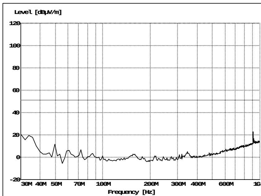
Figure 2. Radiated emission 30 M – 1 GHz, unit UKL 601 04/11.
