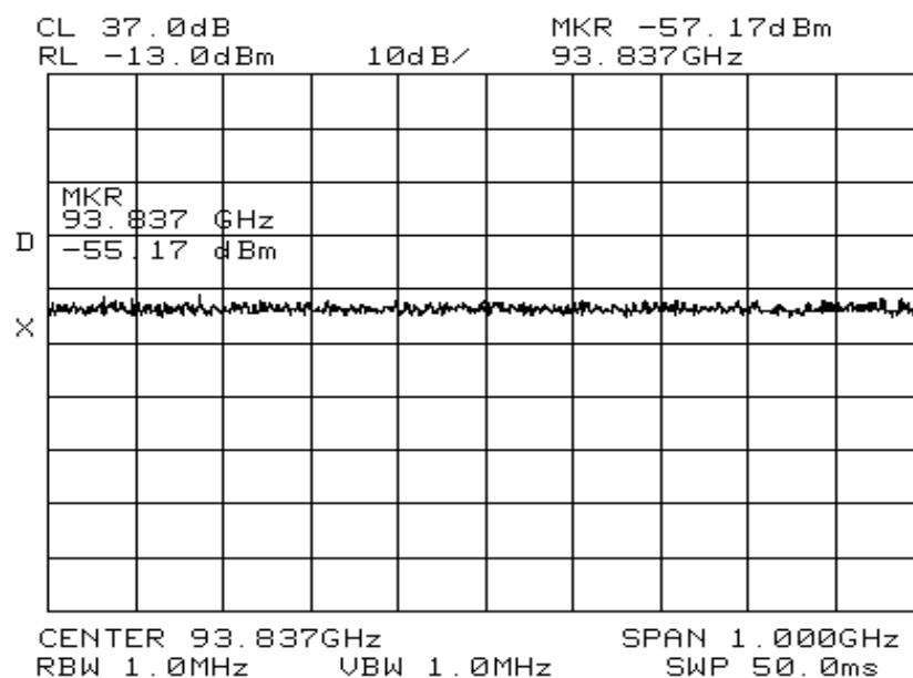
Plot 2 3rd Harmonics
