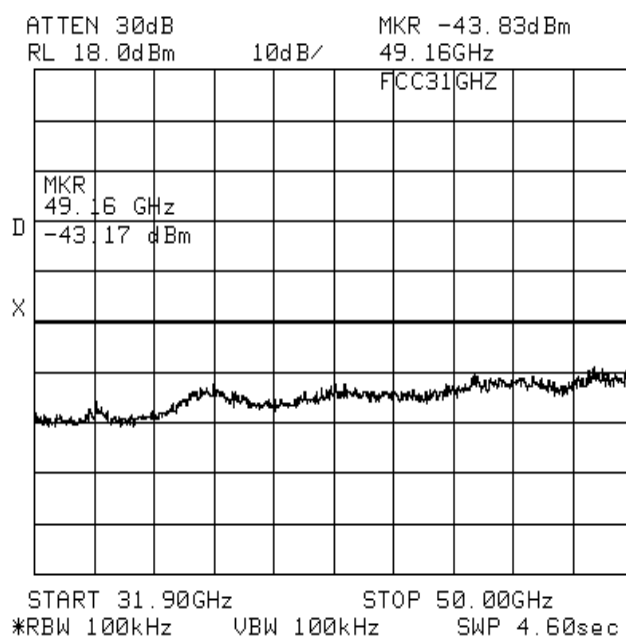
Plot 3 spectrum mask (conducted)
