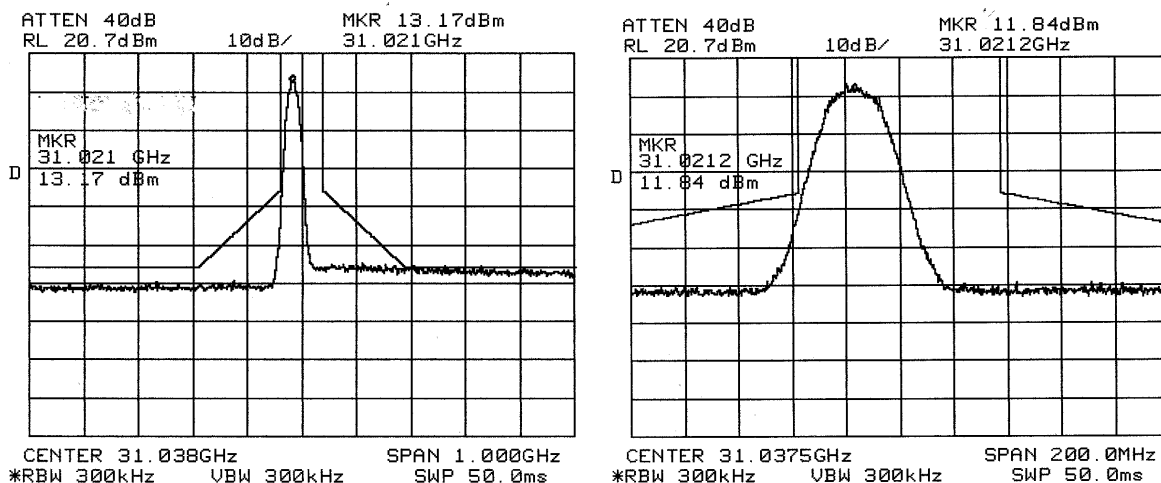
Figure 4-5. 31.021GHz - 1 st channel lower band end measurement.
