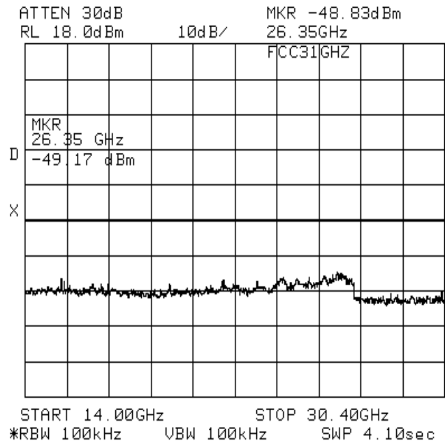
Plot 1 Spectrum mask (conducted)
