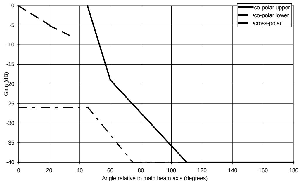
Figure 2.1 Guaranteed azimuth radiation pattern envelope (RPE), Radio node antenna 30 GHz.
