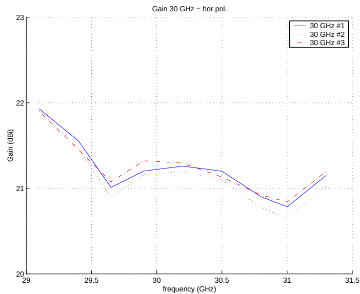
Figure 1 Gain measurements for some horizontally polarized antennas.
