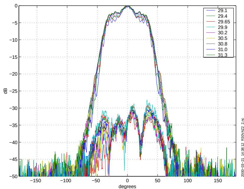
Figure 11 Radiation patterns in azimuth for A23000HUJA.
