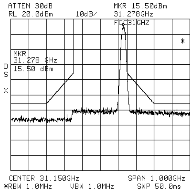
Plot 2 spectrum mask (conducted)
