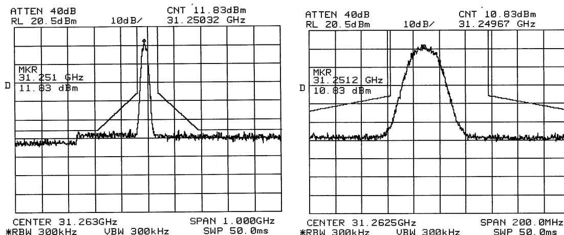
Figure 8-9. 31.251GHz - 1 st channel lower band end measurement.
