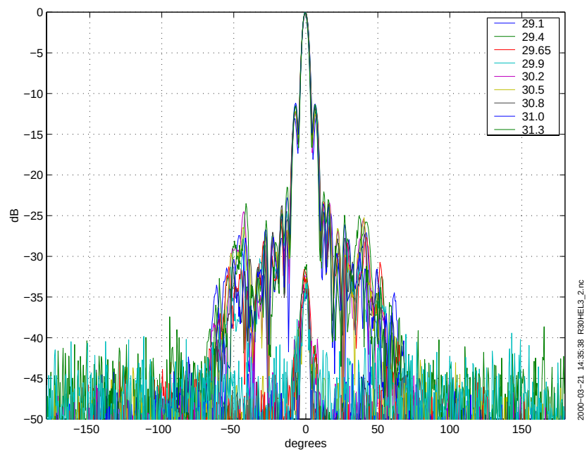
Figure 10 Radiation patterns in elevation for antenna #3.
