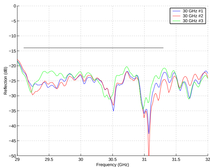
Figure 3 Measured reflection ( S_{11} ) for some horizontally polarized antennas.
