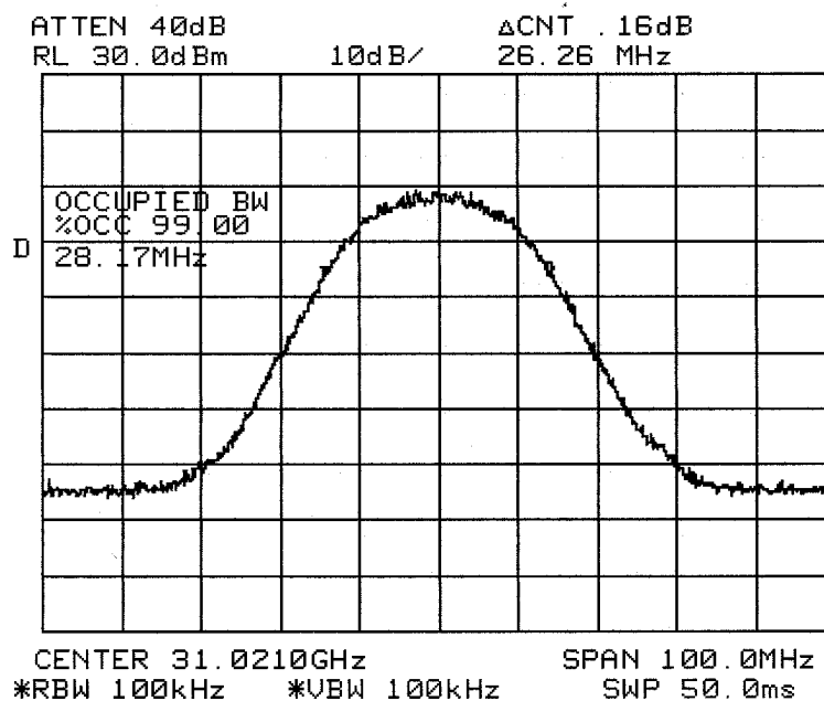
Figure 2- Occupied bandwidth measurement Radio Node UKL 601 04/11
