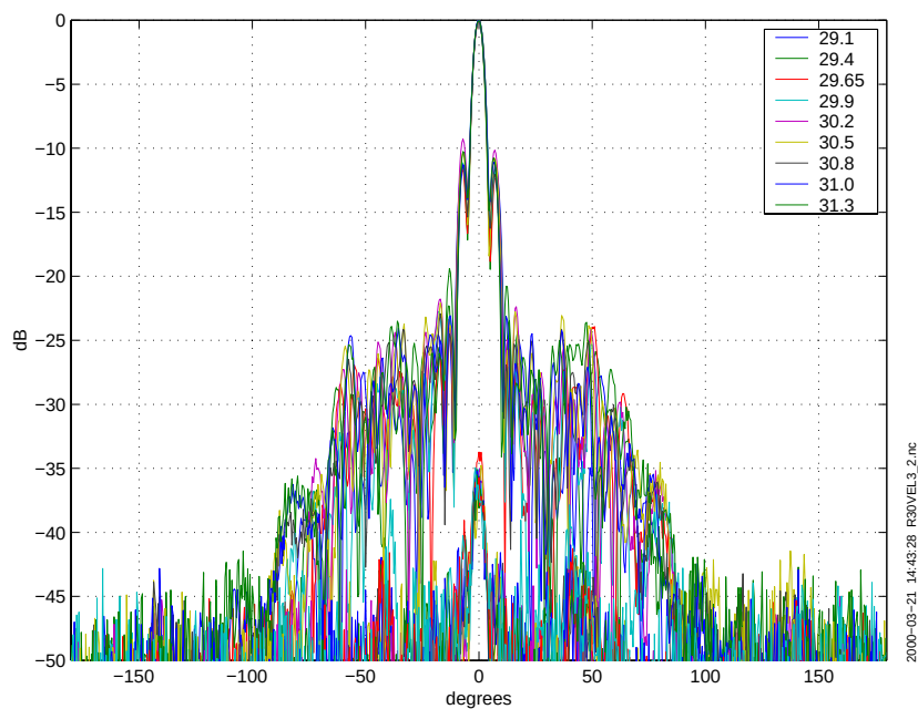
Figure 16 Radiation patterns in elevation for A23000HUJ9.
