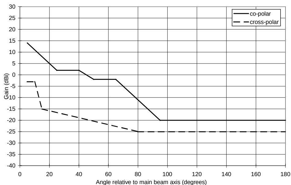
Figure 2.1 Guaranteed radiation pattern envelope (RPE), 0.2 m compact 30 GHz, high performance.
