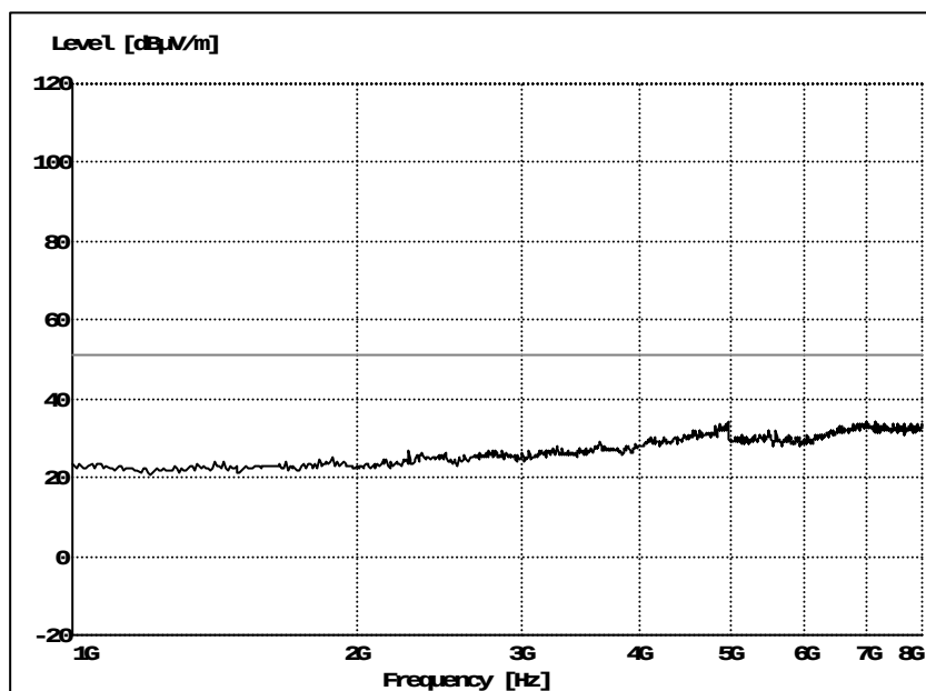
Figure 7. Radiated emission 1 – 8 GHz, Unit UKL 601 04/21
