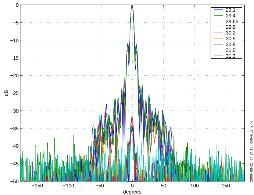
Figure 9 Radiation patterns in elevation for antenna #2.
