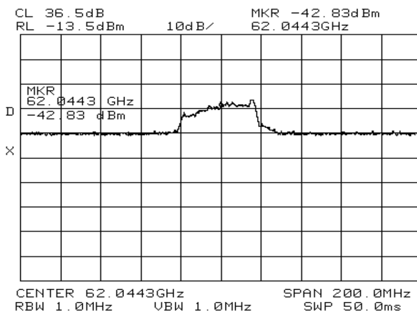
Plot 5 2nd Harmonics
