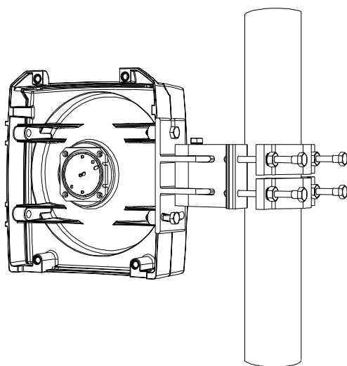
Figure 1.1 0.2 m compact antenna.
