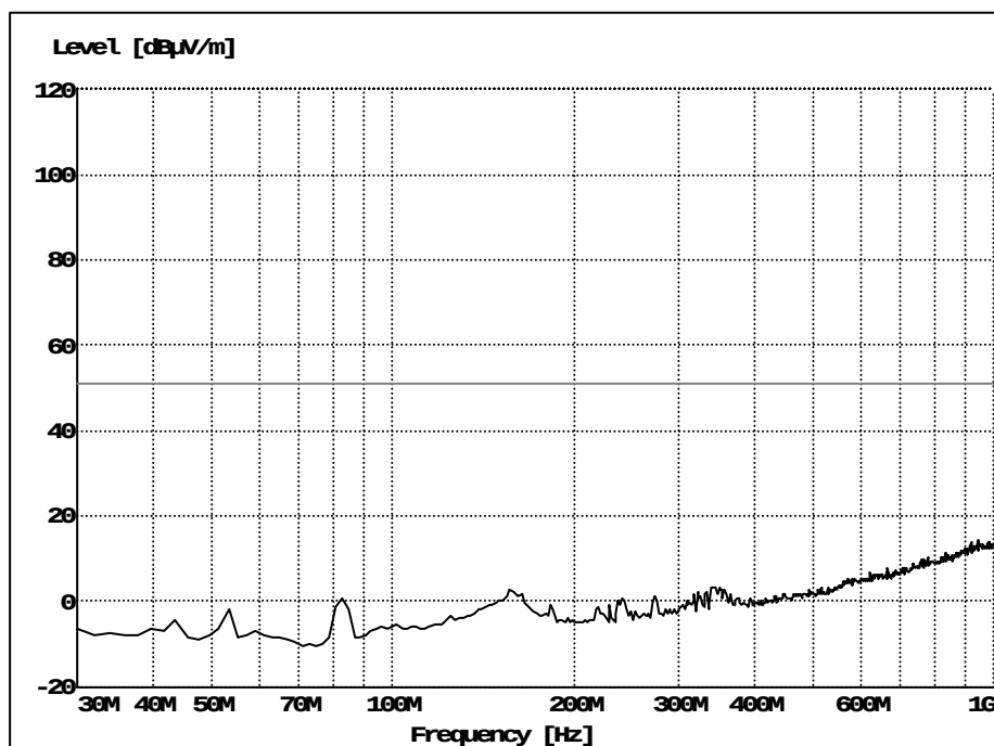
Figure 10. Radiated emission 30 M – 1 GHz, Background measurement. RBW = 3 kHz and VBW = 10 kHz.
