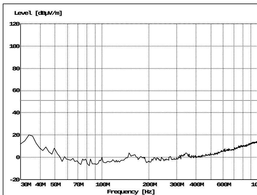
Figure 6. Radiated emission 30 M – 1 GHz, unit UKL 601 04/21
