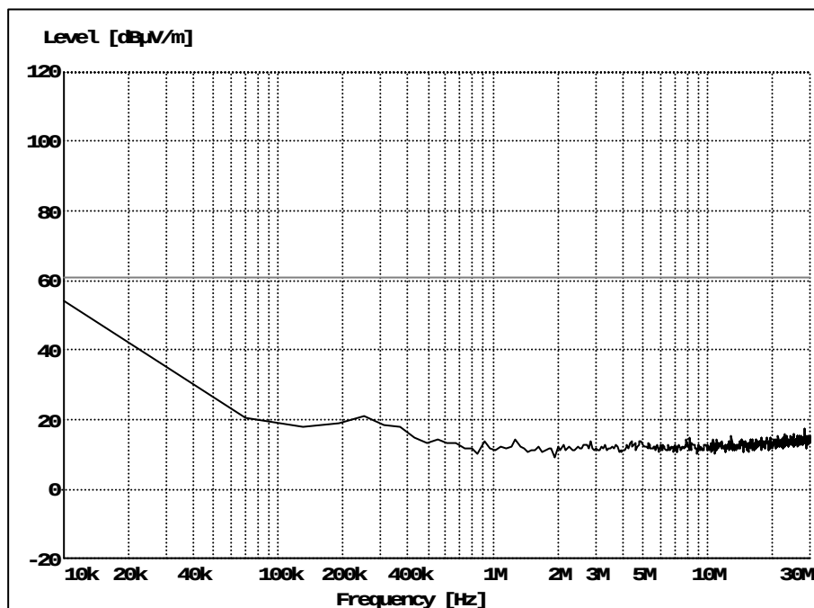
Figure 9. Radiated emission 10 k– 30 MHz, Background. RBW = 3 kHz and VBW = 10 kHz.
