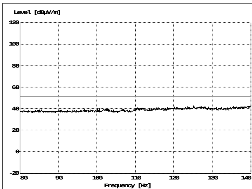
Figure 4. Radiated emission 8 – 14 GHz, Unit UKL 601 04/11
