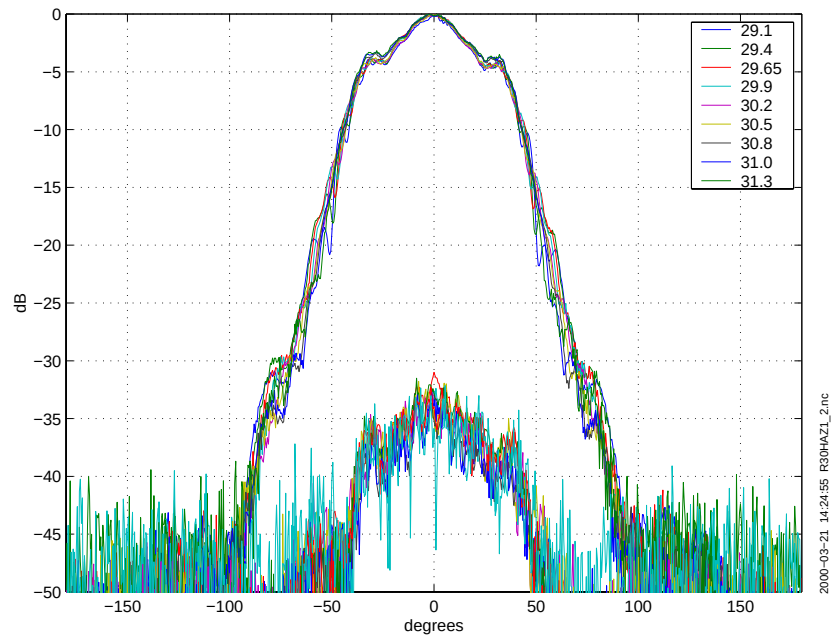
Figure 5 Radiation pattern in azimuth for antenna #1.
