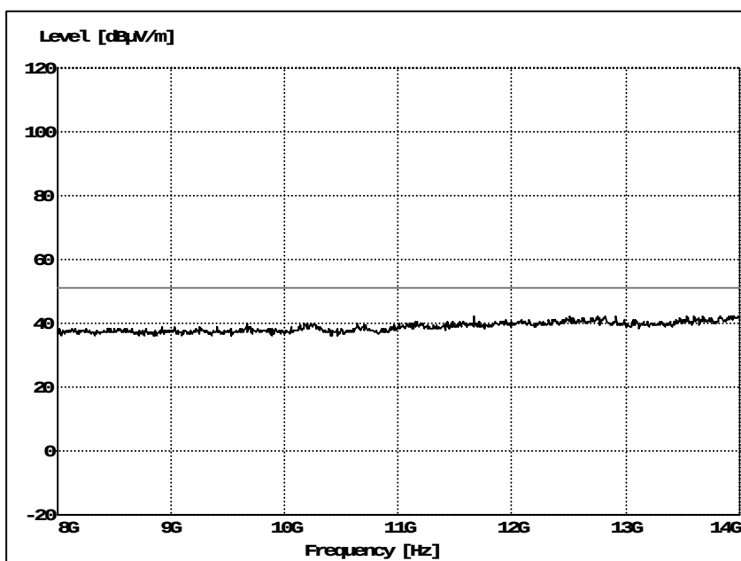
Figure 8. Radiated emission 8 – 14 GHz, Unit UKL 601 04/21
