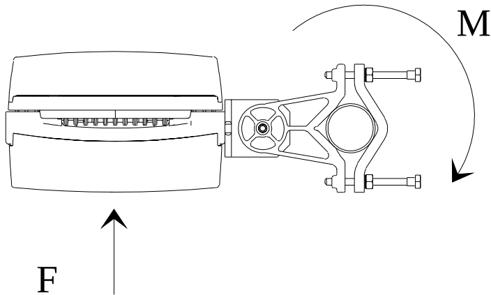
Figure 4.1 Wind load and torque.
