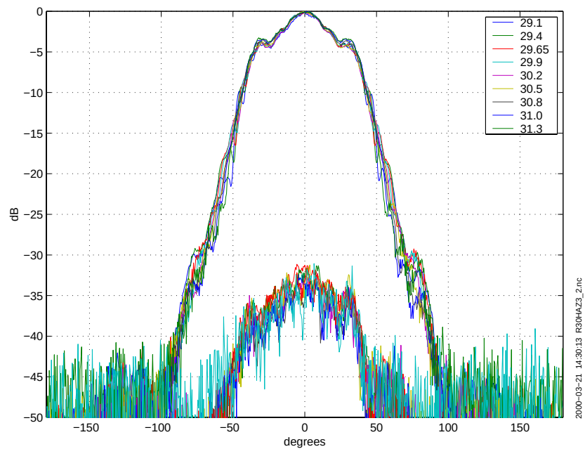
Figure 7 Radiation patterns in azimuth for antenna #3.
