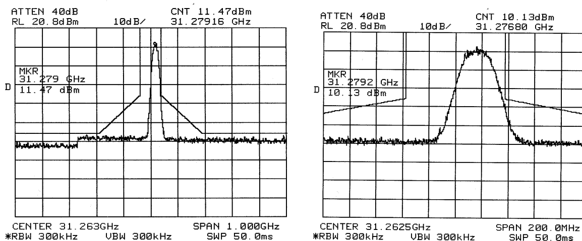
Figure 10-11 31.279GHz - 2 nd channel higher band end measurement.
