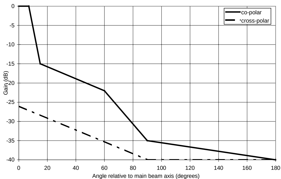
Figure 2.2 Guaranteed elevation radiation pattern envelope (RPE), Radio node antenna 30 GHz.
