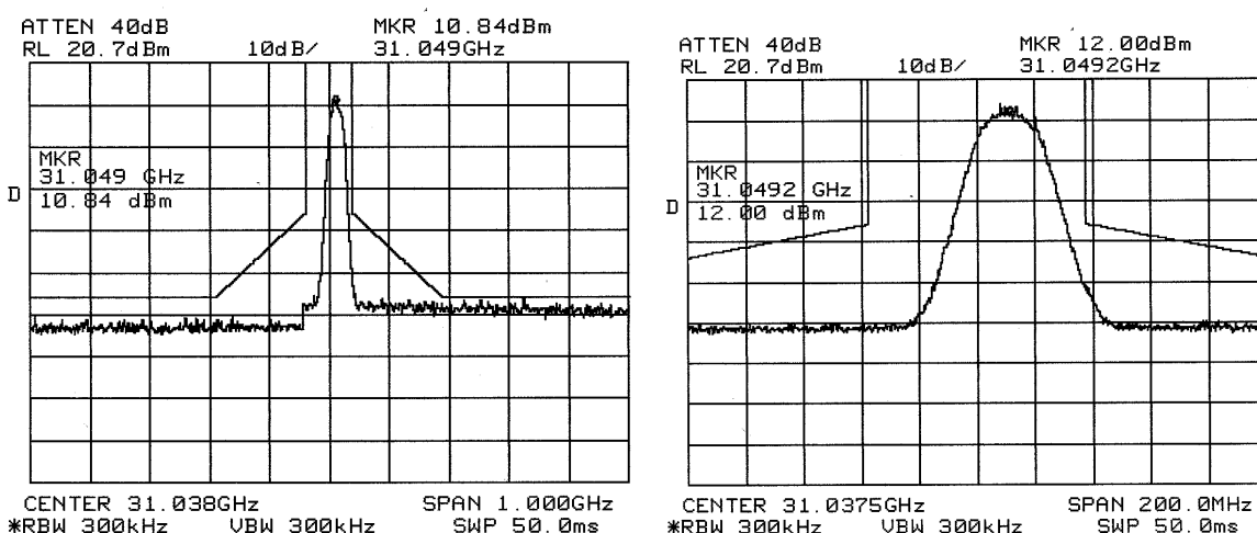
Figure 5-6. 31.049GHz - 2 nd channel higher band end measurement.
