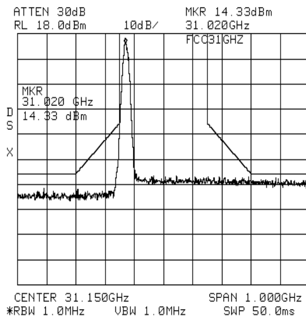
Plot 5 spectrum mask (conducted)
