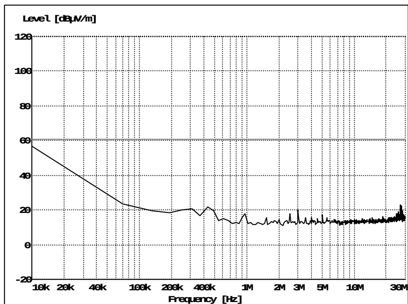
Figure 1. Radiated emission 10 k– 30 MHz, unit UKL 601 04/11.
