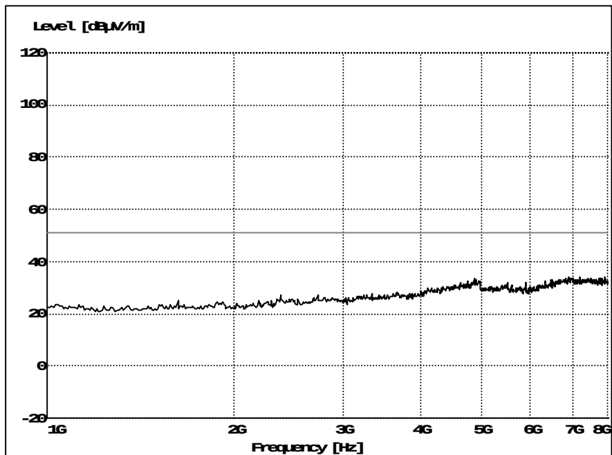
Figure 5. Radiated emission 1 – 8 GHz, Background. RBW = 100 kHz and VBW = 100 kHz.
