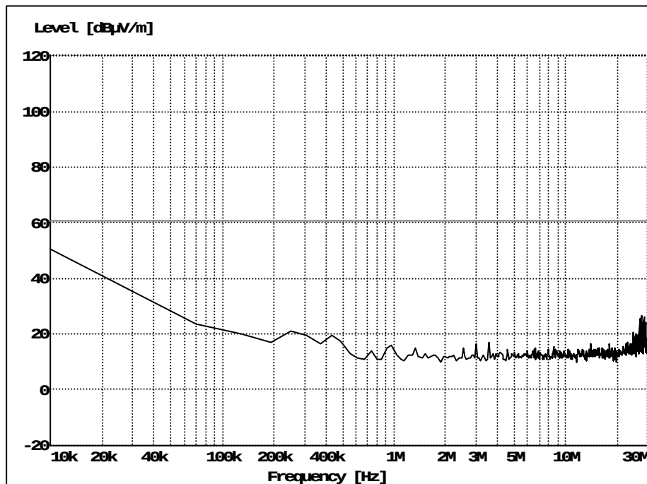
Figure 5. Radiated emission 10 k– 30 MHz, unit UKL 601 04/21
