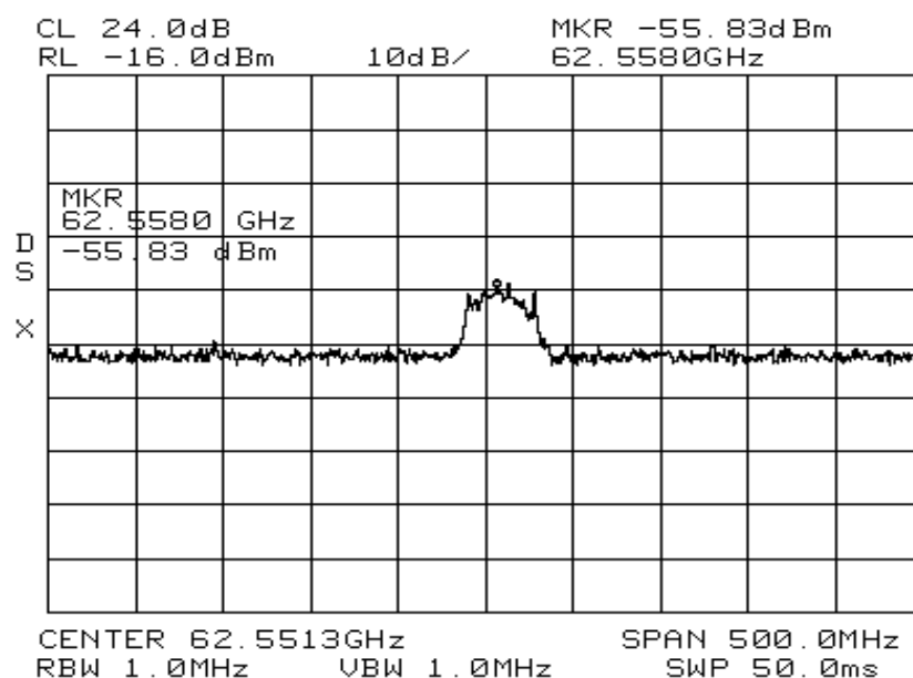
Plot 1 2nd Harmonics
