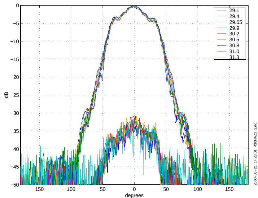
Figure 6 Radiation pattern in azimuth for antenna #2.
