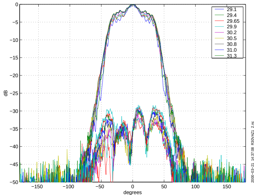
Figure 11 Radiation patterns in azimuth for A23000HUJA.
