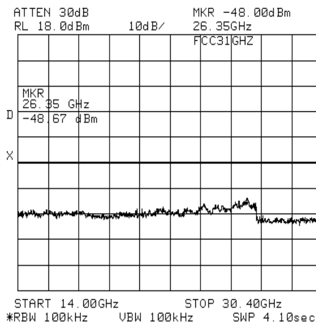
Plot 4 spectrum mask (conducted)
