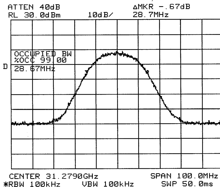
Figure 3- Occupied bandwidth measurement Radio Terminal UKL 601 04/21
