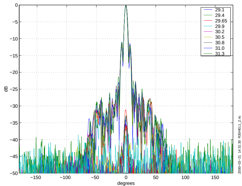
Figure 8 Radiation patterns in elevation for antenna #1.
