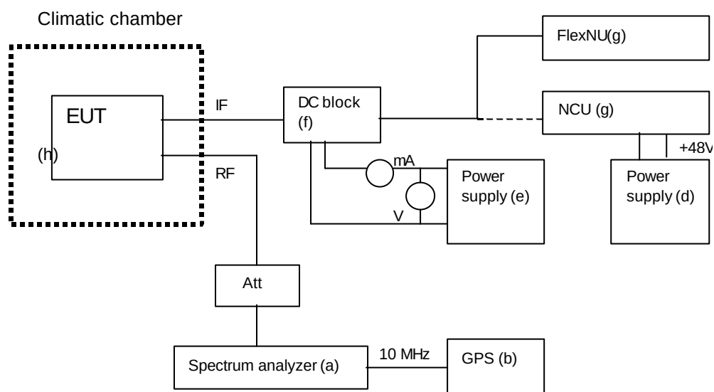
Figure 1 – Sketch of measurement set-up
