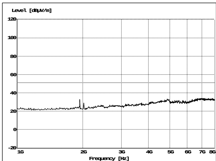
Figure 3. Radiated emission 1 – 8 GHz, Unit UKL 601 04/11
