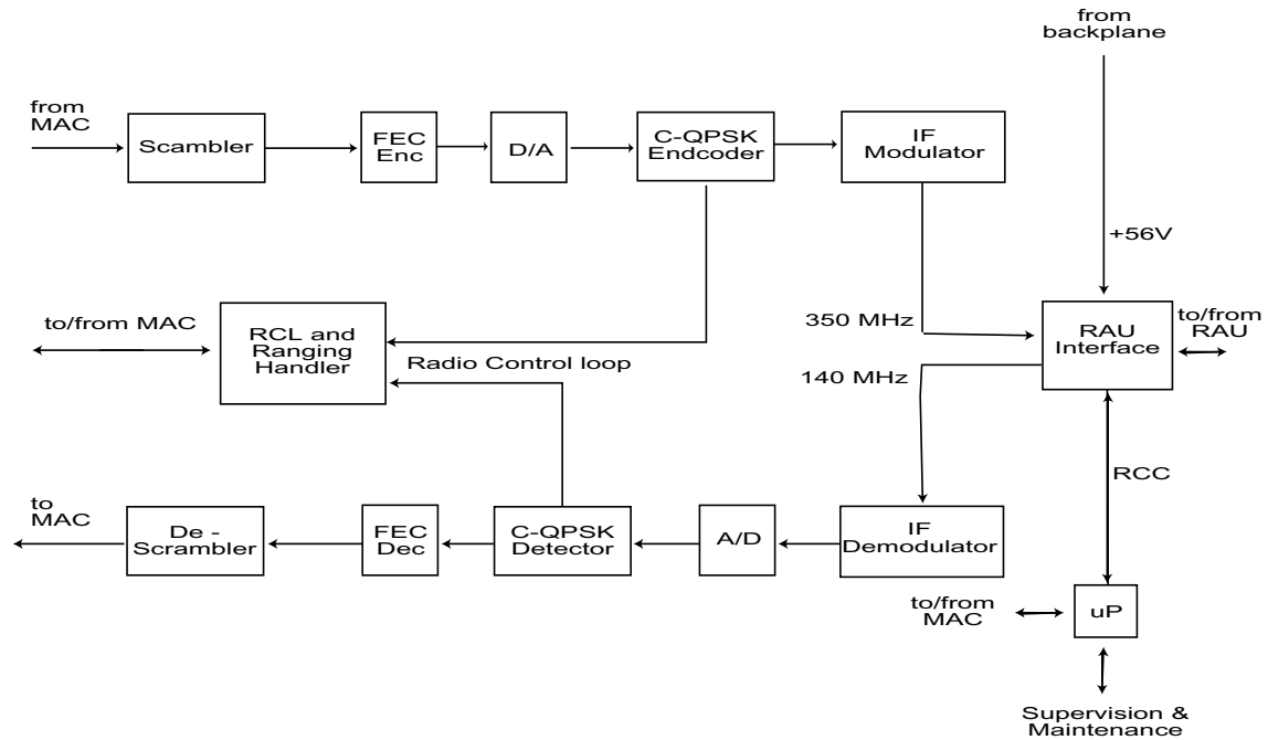
Figure 5-3 Modem Board Functional Block Diagram
