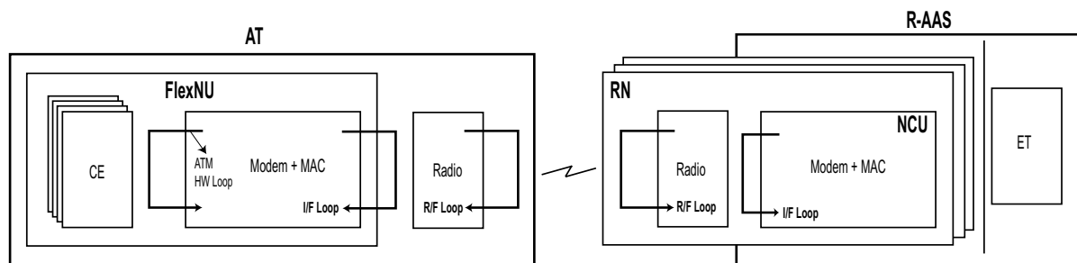
Figure 9-2 RN Near-End Loops and AT Near-End Loops
