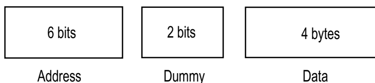
Figure 5-14 RC Frame Format
