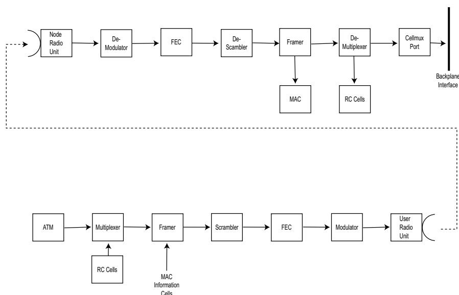
Figure 5-13 Block Diagram for the Uplink Stream
