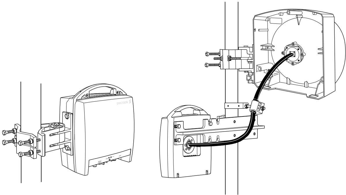
Figure 8-3 RAU Fitted Directly and Separately to the Antenna
