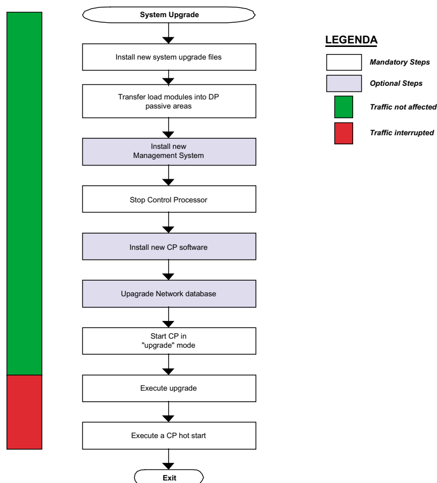
Figure 9-3 System Upgrade
