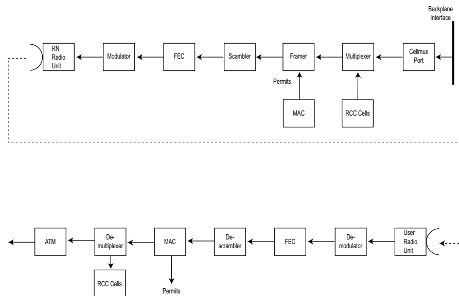
Figure 5-12 Block Diagram for the Downlink Stream
