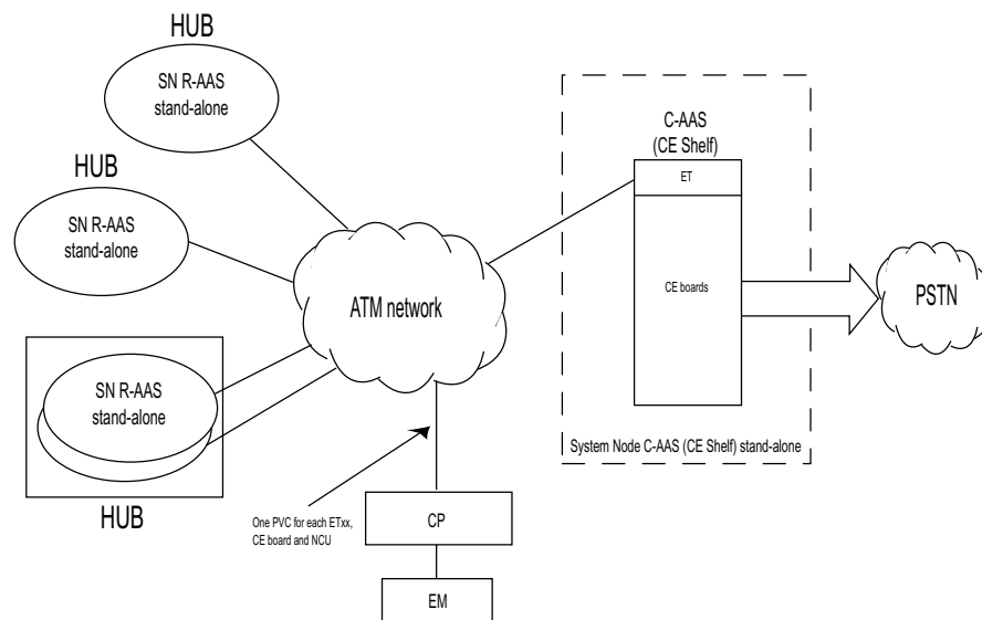
Figure 3–2 SN C-AAS Stand-Alone
