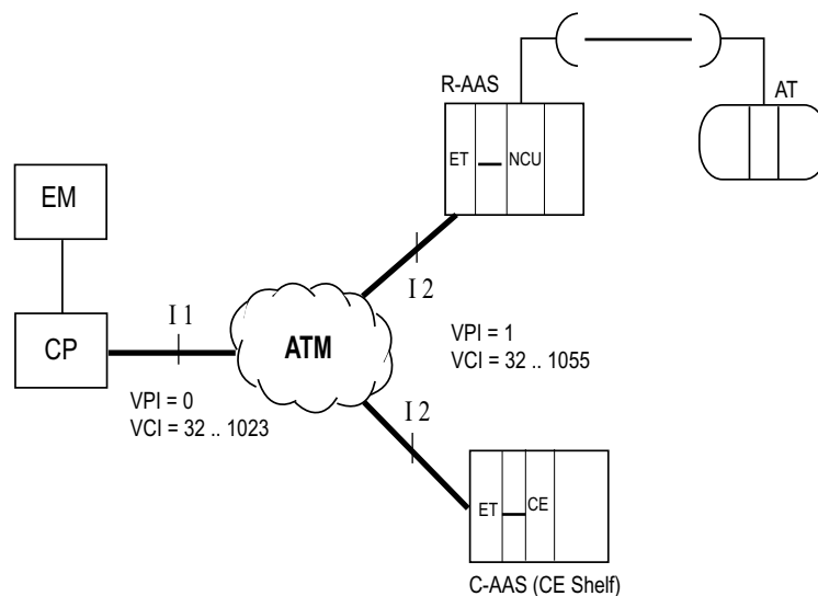
Figure 6-4 I1 and I2 Interfaces
