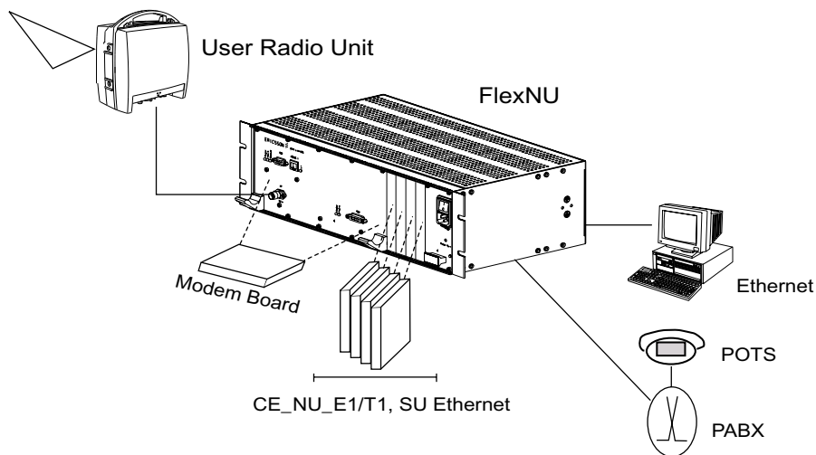
Figure 2-3 AT
