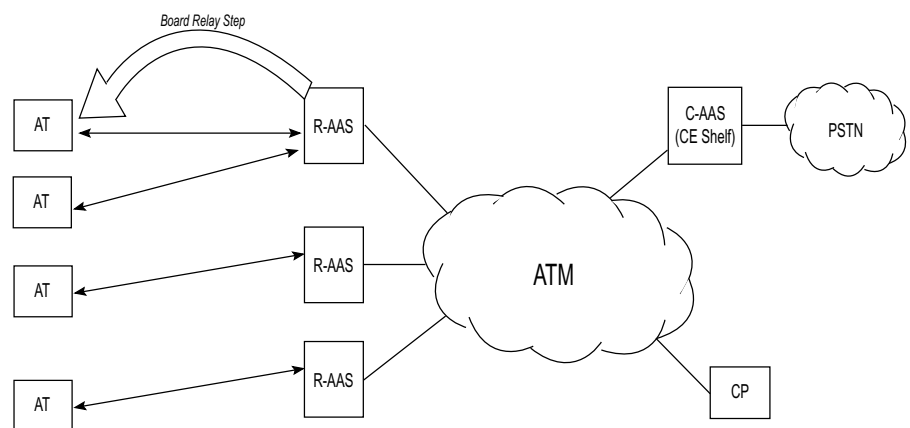
Figure 6–3 Board Relay Steps: Correct Configuration
