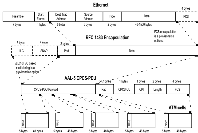
Figure 4-3. Ethernet Frame Encapsulation on ATM in the AT
