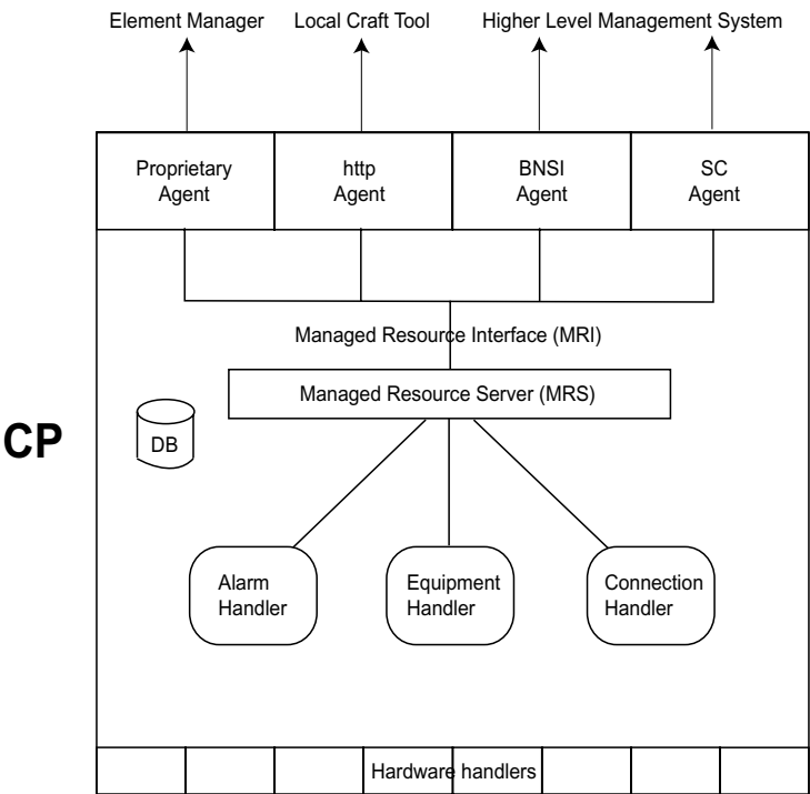
Figure 6-8 CP Software Architecture, Functional View
