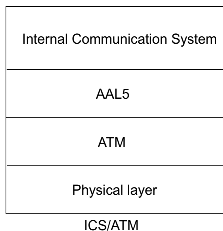
Figure 6-10 ICS over ATM.
