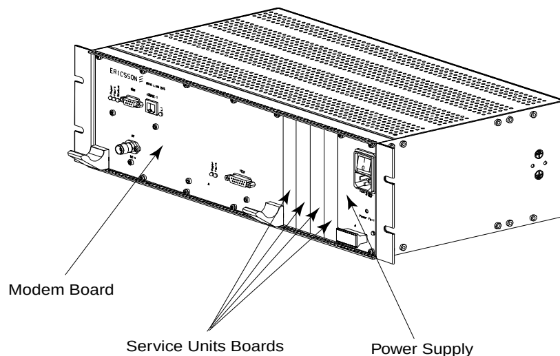
Figure 8-7 The FlexNU Indoor Unit
