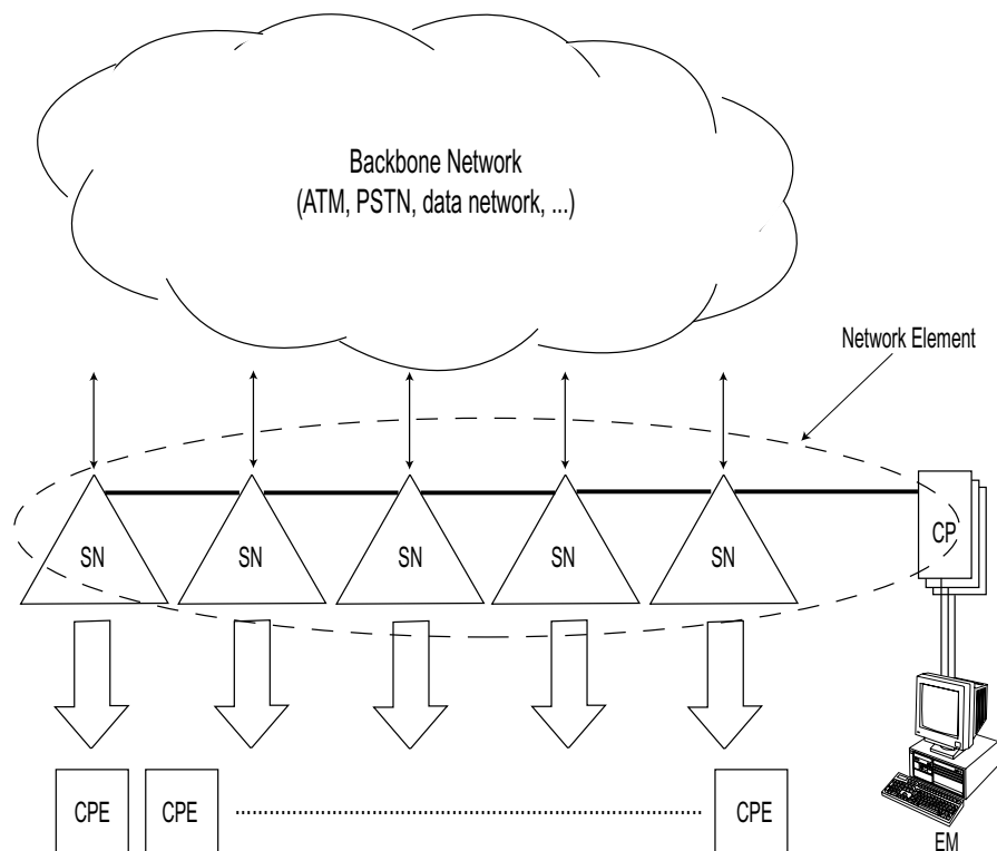
Figure 3-3 Generic MINI-LINK BAS Network
