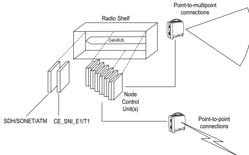
Figure 2-6 R-AAS
