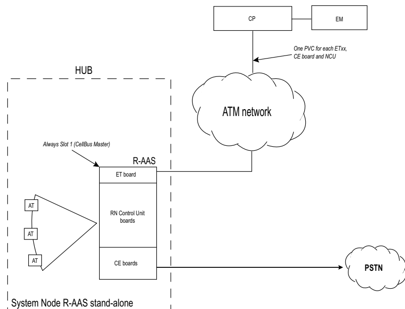
Figure 3-1 SN R-AAS Stand-alone
