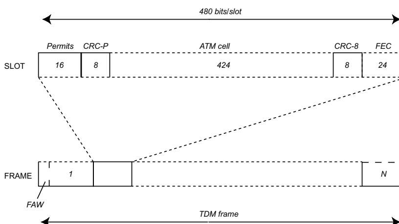
Figure 5-6 Downlink TDM Frame
