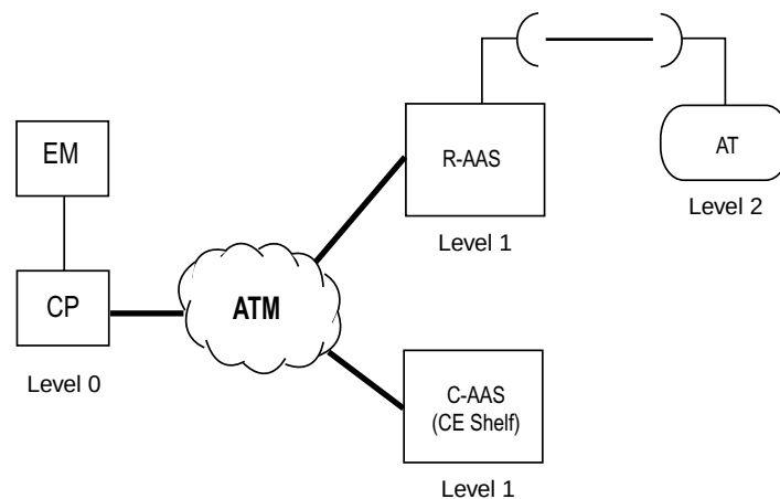
Figure 6-2 Control Architecture Levels
