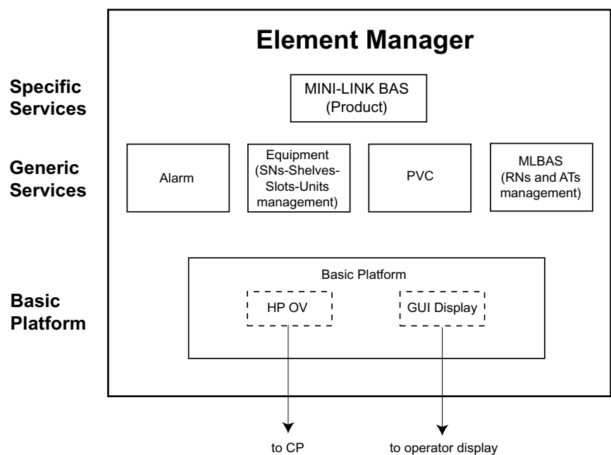
Figure 6-5 EM Software Architecture
