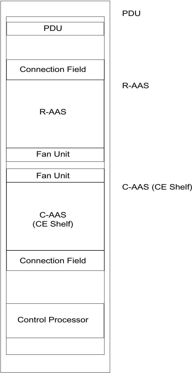
Figure 8-15 Central Office in Cabinet BYB 501
