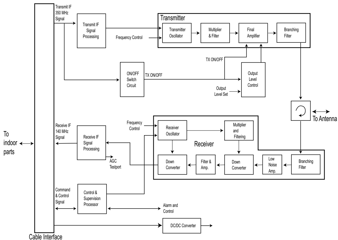
Figure 5-5 General RAU Block Diagram
