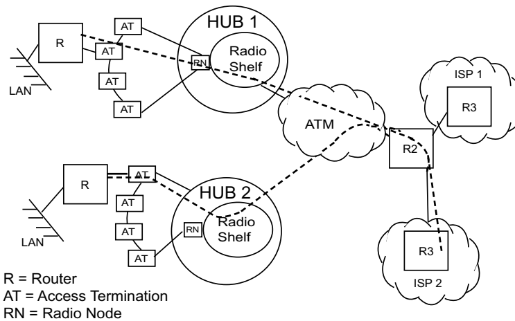
Figure 3-10 System Deployed for Data Traffic and Multiple IP Selection
