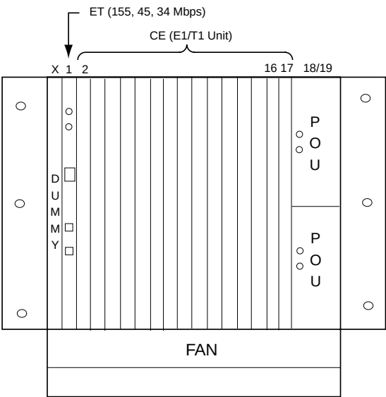
Figure 8-9 C-AAS (CE Shelf) Rear Access Type
