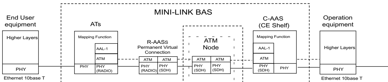
Figure 4-4. OSI Model for Transparent Transport of E1/T1 Data in MINI-LINK BAS
