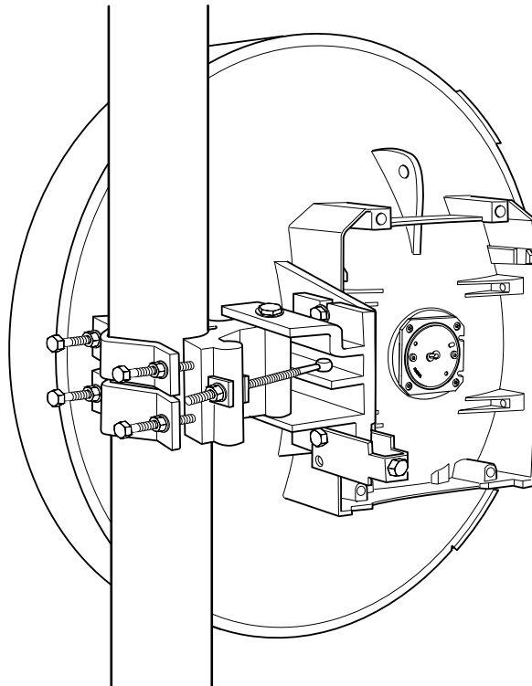
Figure 8-6 0.60 m Integrated Standard Directive Antenna
