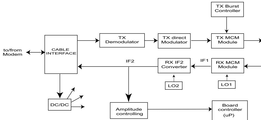
Figure 5-2 Radio Board Functional Block Diagram
