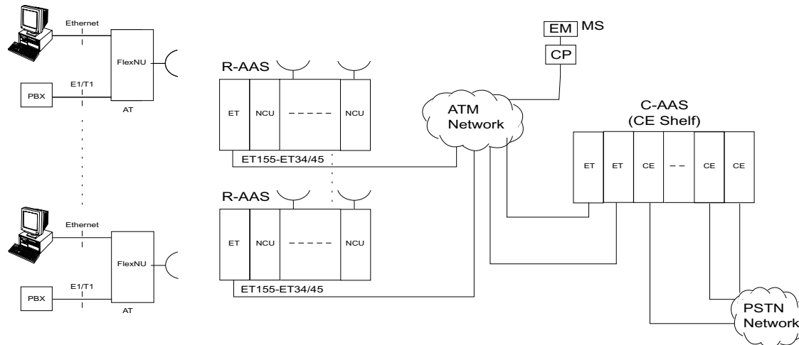
Figure 3-5 Network Example with R-AAS and C-AAS
