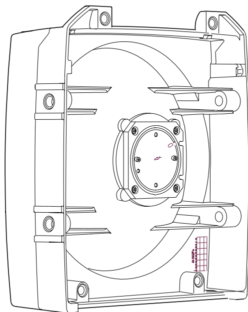
Figure 8-5 Standard Compact Directive Antenna
