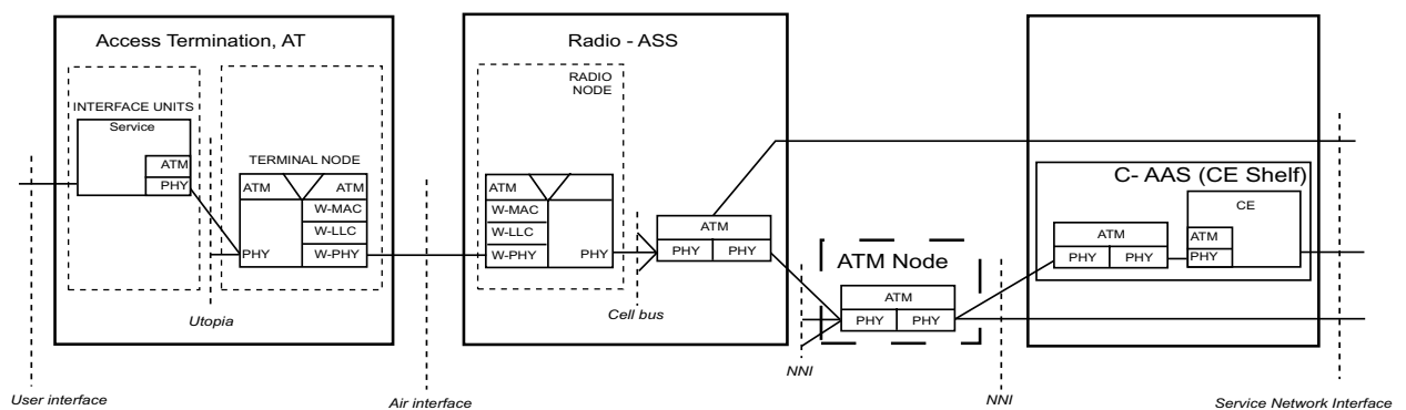
Figure 5-1 Generic MINI-LINK BAS System Model
