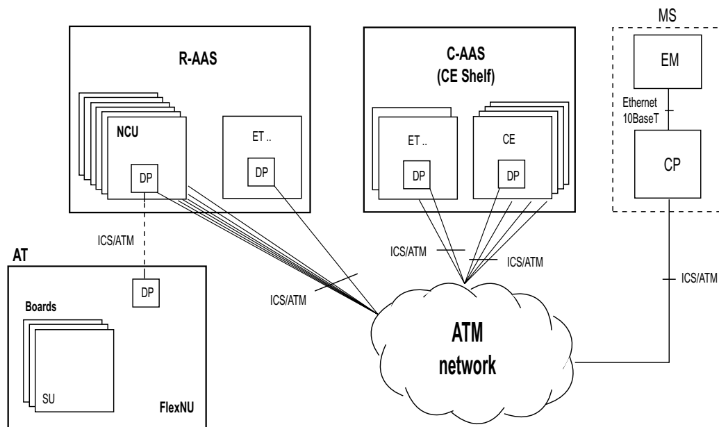
Figure 9-1 MINI-LINK BAS Control Architecture
