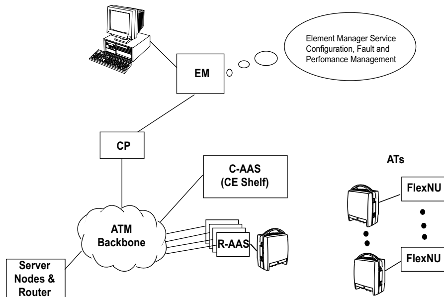
Figure 2-1 MINI-LINK BAS Generic Network
