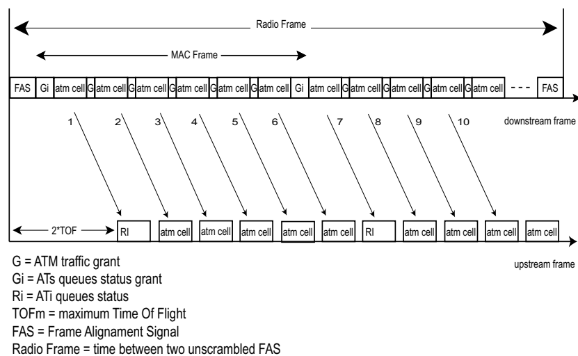
Figure 5-8 Up-Stream and Down-Stream Frames
