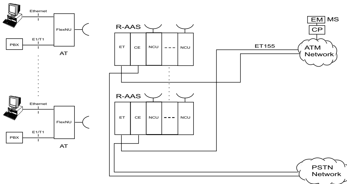
Figure 3-6 Network Example with R-AAS
