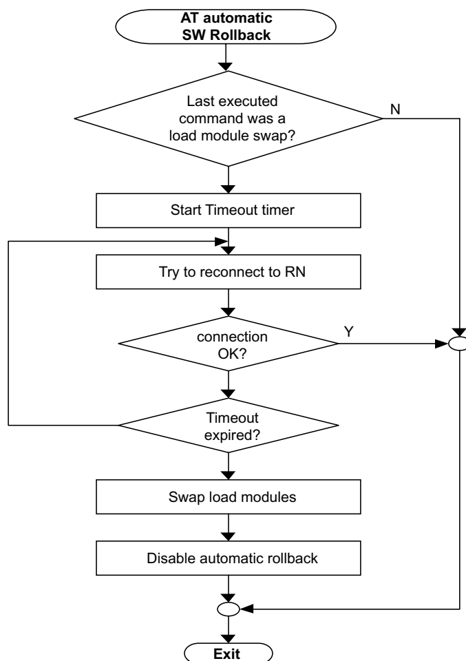
Figure 9-5 Automatic SW Rollback in the AT
