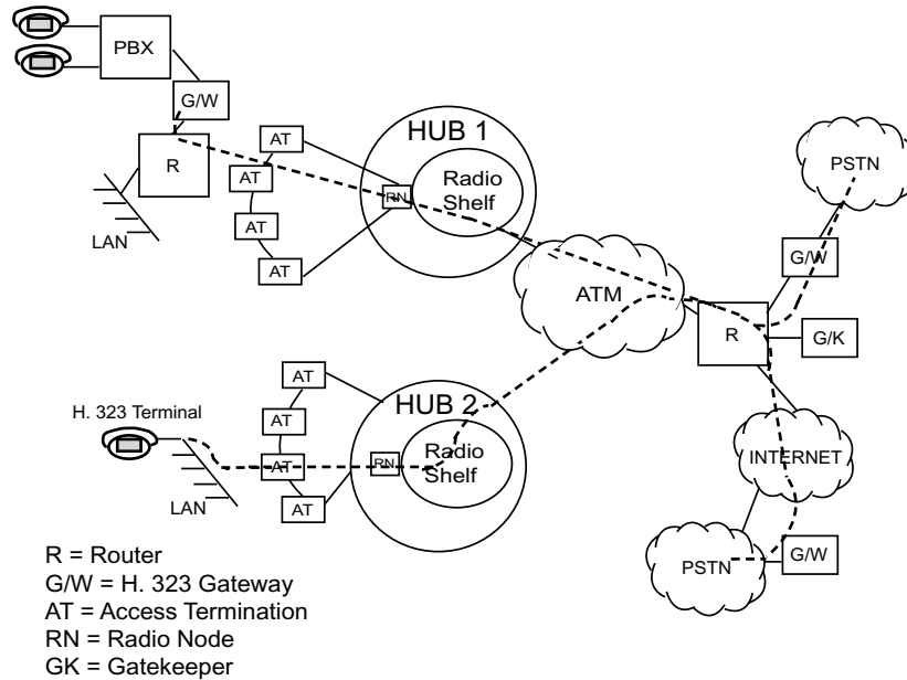
Figure 3-9 System Deployed for IP Telephony (PBX-PSTN, PBX-H.323 terminal)
