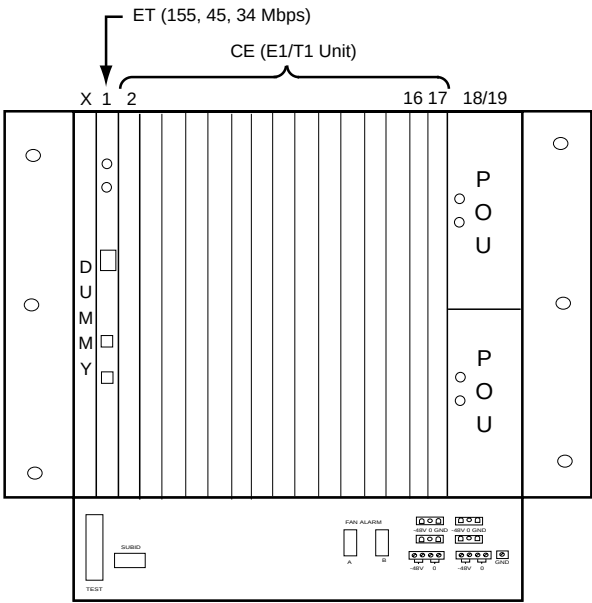
Figure 8-8 C-AAS (CE Shelf) Front Access Type
