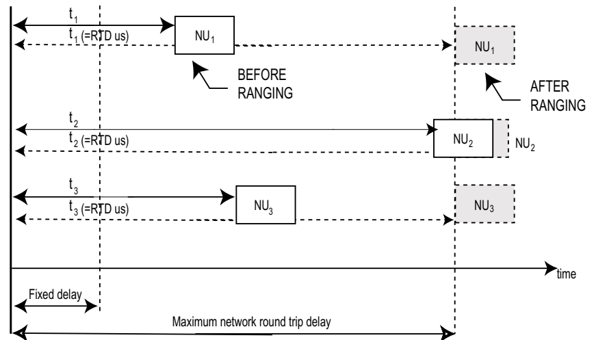
Figure 5-11 Distance Ranging Procedures
