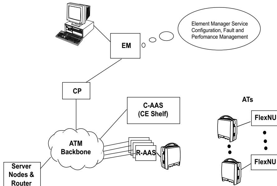
Figure 6-1 Management System Architecture
