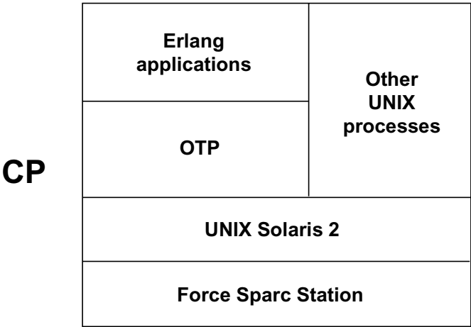
Figure 6-7 CP Software Architecture, Structural View
