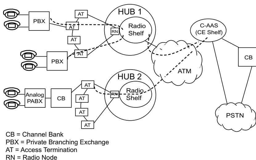
Figure 3-8 System Deployed for Telephony (PBX-PSTN, PBX-PBX)
