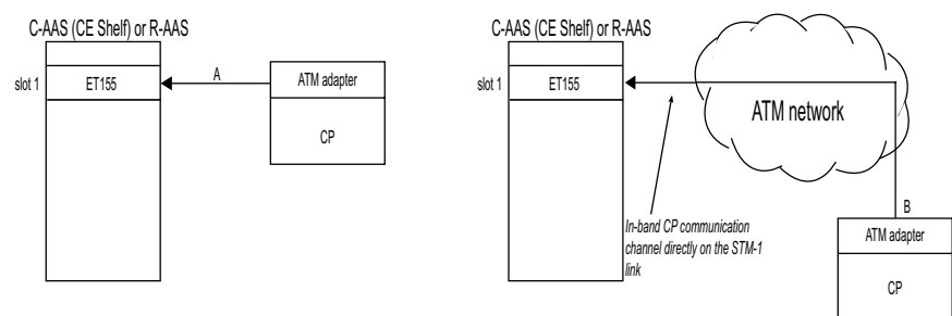
Figure 3–4 CP-SN Connection through ATM Network
