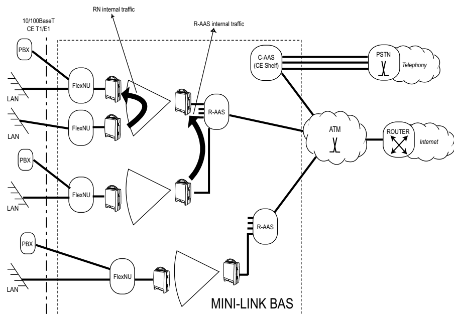
Figure 3-7 MINI-LINK BAS with AT-to-AT Connections
