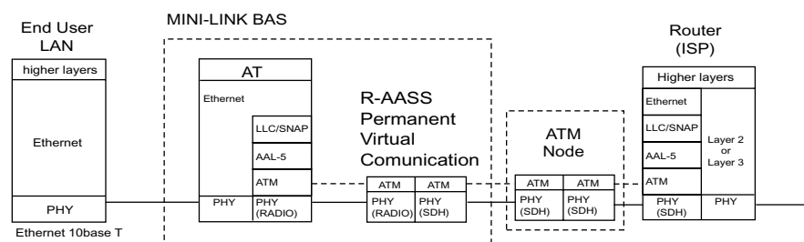
Figure 4-2. Protocol Stack Model for Ethernet Frames in MINI-LINK BAS
