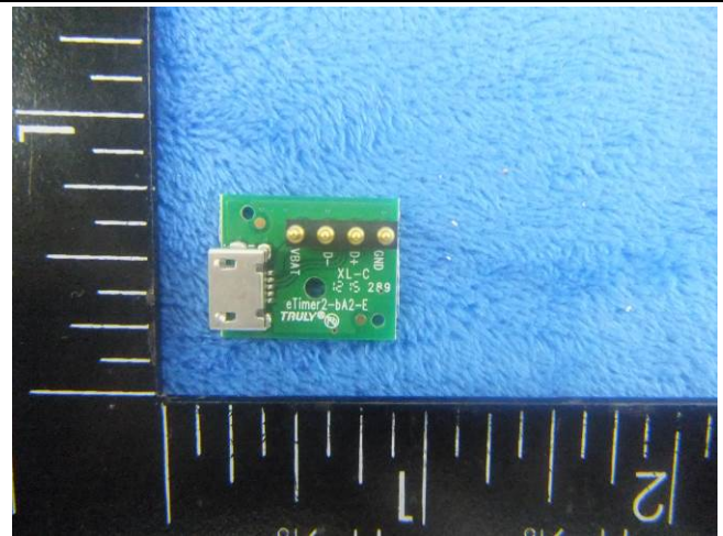
USB Adapter board - Front View
