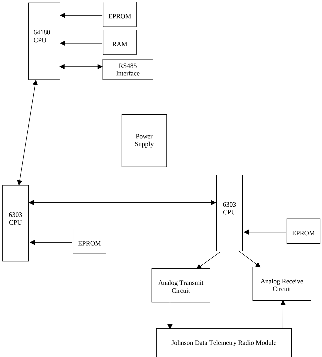
RBSIII Block Diagram
