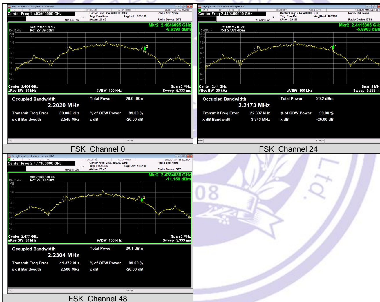
99% Bandwidth
