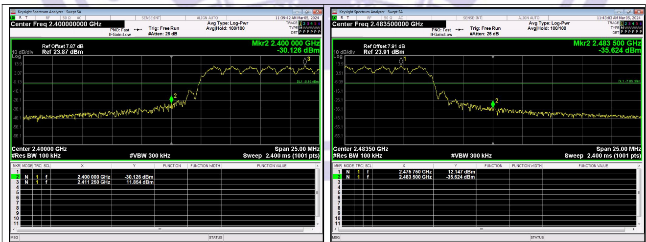
Out Of Band Emission(Left) FSK_Channel Hopping
