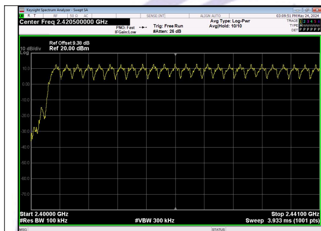
Low End Spectrum Channel Hopping Plot FSK
