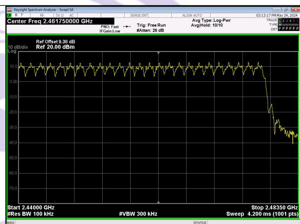
High End Spectrum Channel Hopping Plot FSK
