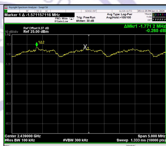
FSK_Channel 24
