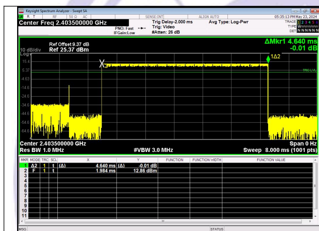
Pulse Width
