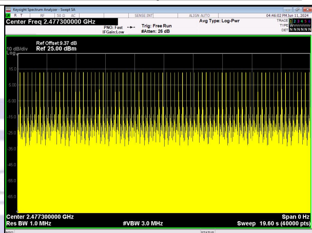
Number of Pulses in 19.6 seconds
