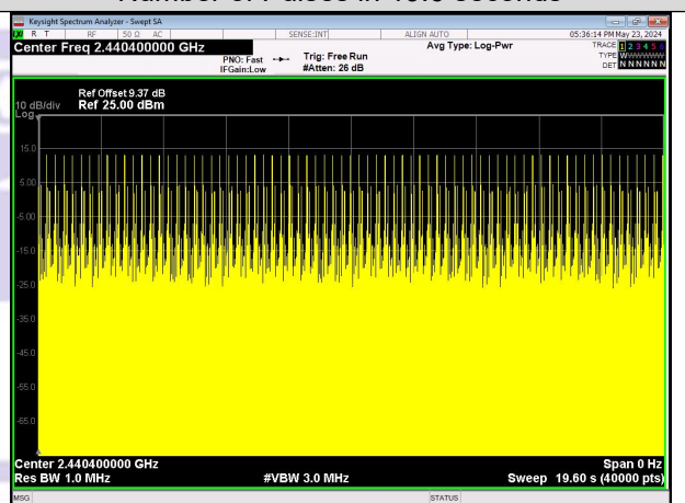
Number of Pulses in 19.6 seconds
