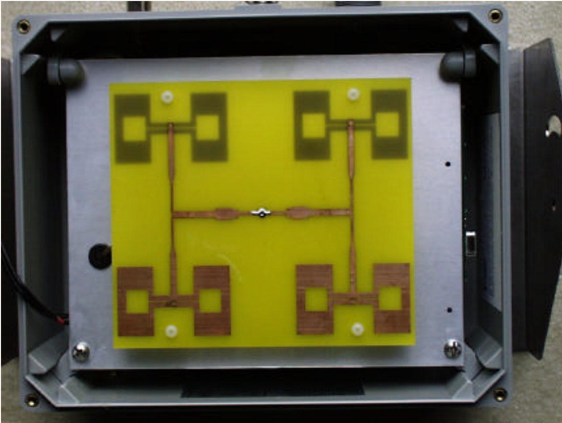
Top view, lid open, showing built-in antenna
