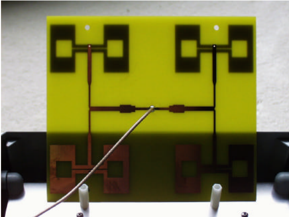
Built-in antenna, detail, showing coax connection
