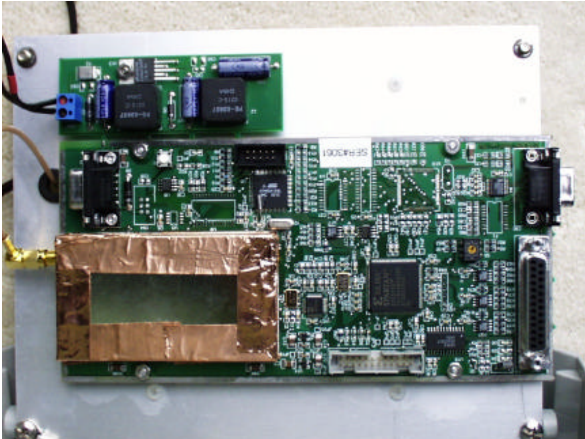
EUT pcb board, top view
