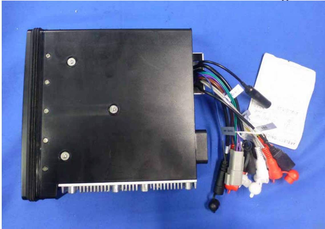
Figure 7 General Appearance of the EUT
